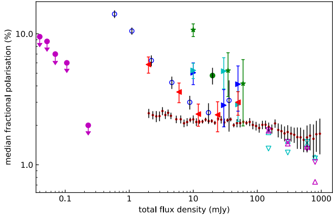
Fig. 9. Median fractional polarisation over total intensity for different catalogues. The red dots give the data points of Stil et al. (2014) , who used the NVSS catalogue and a stacking technique, and the open turquoise upward (steep) and downward (flat) pointing triangles are the polarised sources from Tucci et al. (2004) of the NVSS split up by a spectral index of -0.5 . The open magenta triangles represent the sources from Mesa et al. (2002) split by the same spectral index limit. The magenta circles represent upper limits from the catalogue of Rudnick & Owen (2014) . The green stars are from Grant et al. (2010) , the green circle from Taylor et al. (2007) , and the blue open circles from Subrahmanyan et al. (2010) . The triangles pointing to the right are the data from Hales et al. (2014a) , the blue ones represent their data for the ELAIS-S1 field, and the turquoise ones their data for the CDF-S field. The red triangles pointing left represent our polarised sample.
