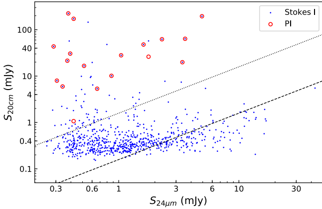
Fig. 4. Radio flux density compared to FIR flux density for all sources with a 24\ \mu\text{m} counterpart. The red circles indicate the 18 polarised sources with a 24\ \mu\text{m} counterpart. The dashed line gives the FRC from Appleton et al. (2004), and the dotted line indicates the radio flux density being ten times greater than for the FRC.
