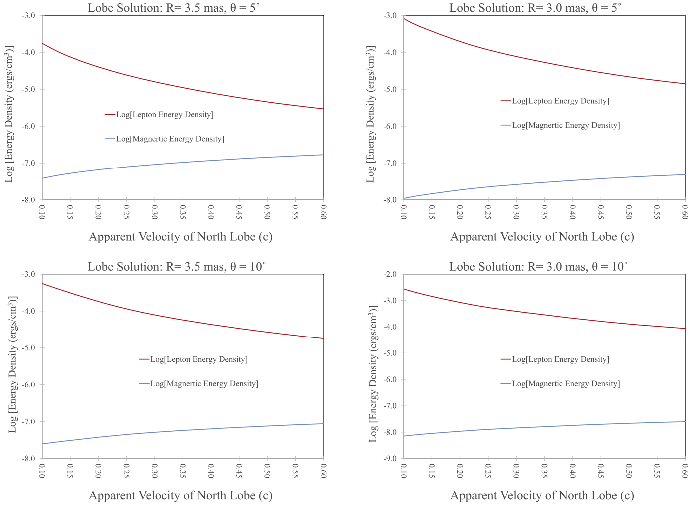
Figure 14. This figure explores a large subset of the solution space for a spherical plasmoid that radiates the fit to the north lobe (Figure 13). Based on Equations (10) and (12), we choose a rectangular subset 3.0 \text{ mas} < R < 3.5 \text{ mas} and 5^\circ < \theta < 10^\circ and bound its behavior by looking at the four corners of the rectangle. By plotting U_e and U_B as a function of \beta_{\text{app}} , we find no solutions that are near equipartition and obey the upper bound on \beta_{\text{app}} from Equation (11). The closest solution to equipartition is at R = 3.5 \text{ mas} and \theta = 5^\circ in the upper-left panel.
