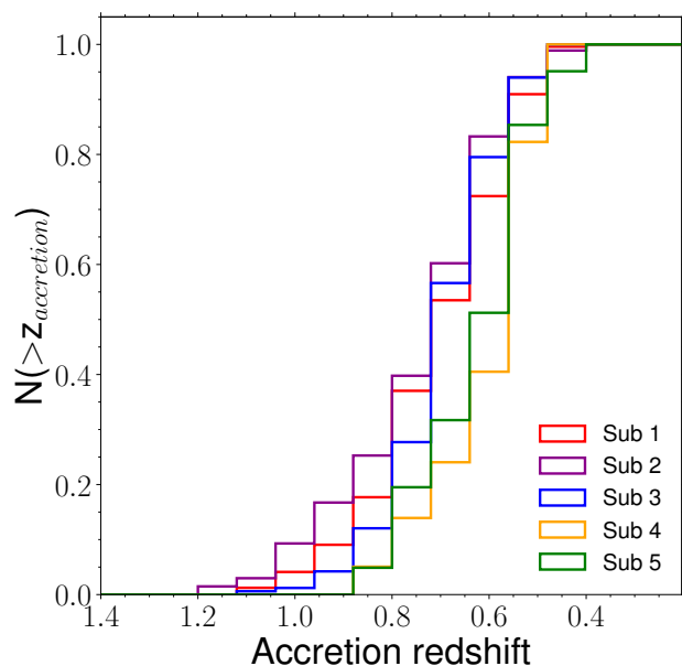
Fig. B.3: Cumulative distribution of accretion redshift for galaxies belonging to the five sub-clumps.
