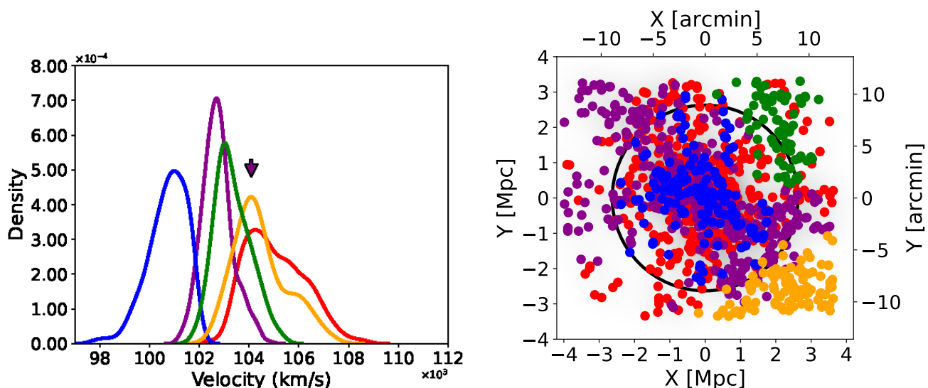
Fig. B.1: Velocity ( Left panel ) and 2D ( Right panel ) distributions of the 5 substructures detected with 3D-DEDICA. The arrow indicates the velocity of the BCG. The colour-code, velocity peak, and the centre for each substructure are reported in Tab. B.1. In the right panel, the circle has a radius equal to r_{200} = 2.63 Mpc.
