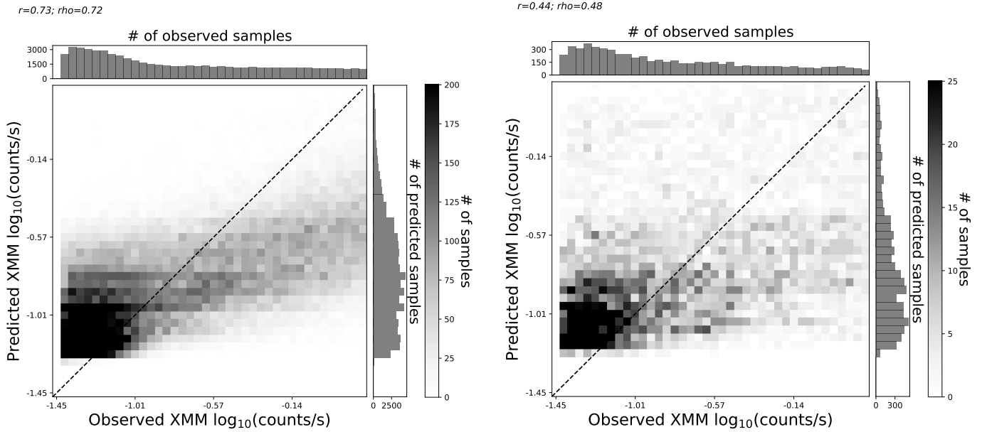
Figure 7. Observed count rates from the trained (left) and test (right) data set versus those predicted by the model. The color represents number of samples.
