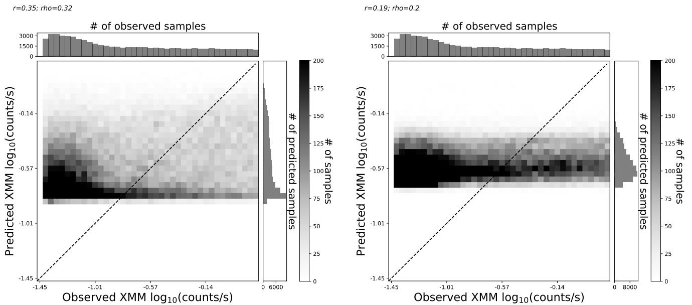
Figure 10. Observed count rates from the trained data set versus those predicted by the linear models: depending on ZGSE (left) and VxSW\_GSE (right). The color represents number of samples.
