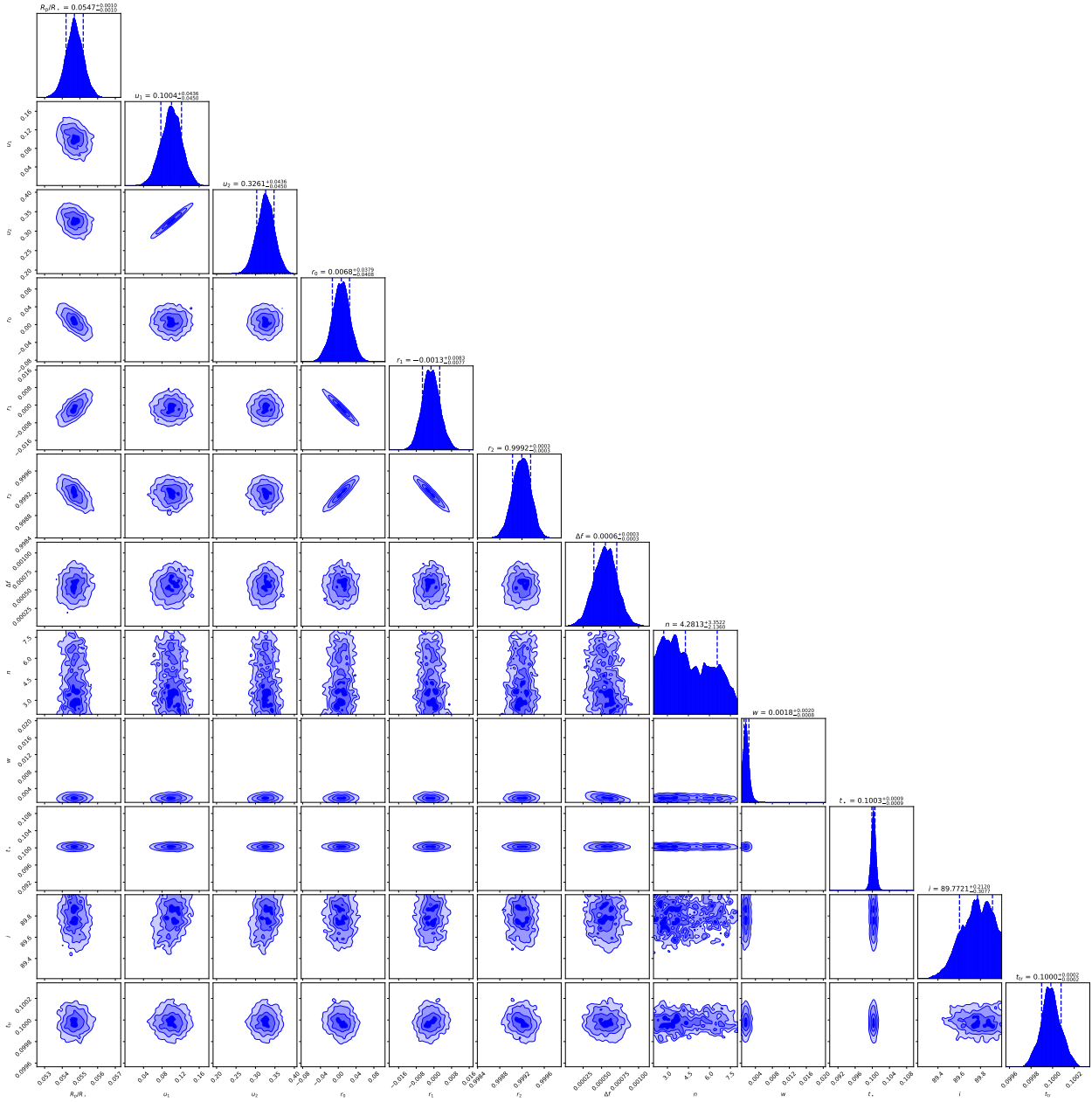
Figure A1. Marginalised posterior distributions for the low-SNR, white-light transit nested sampling on a 14.5 K mag, M star observed with NIRSpect/Prism and a T_{\text{oc}} = 3200 K occulted starspot, with \theta = 0^\circ , as discussed in Section 4.3. The columns represent, from left to right: planet-to-star radius ratio, linear and quadratic limb darkening coefficient, out-of-transit quadratic trend parameters ( r_0 , r_1 , r_2 ), flux bump \Delta f , occultation flatness n , spot width w , occultation time t_* , spot latitude l , and transit mid-time. On large-SNR occultation cases, the n parameter is tightly constrained.
