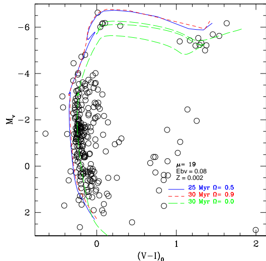
Figure 5. Color-magnitude diagram of NGC 330. The isochrone at 30 Myr is obtained from the Padova and TRieste Stellar Evolution Code (PARSEC; Bressan et al. 2012; Marigo et al. 2017) (the green long-dashed line); the isochrones computed from rotating stellar models at 25 Myr with \omega = 0.5 \omega_c (blue line), and at 30 Myr with \omega = 0.9 \omega_c (red dashed line) are taken from Georgy et al. 2014. The adopted values for the age, distance modulus, reddening, and metallicity are quoted in the figure.
