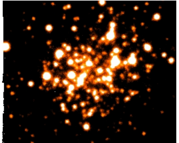
Figure 1. MUSE image of NGC330 at \lambda \sim 4800 Å. North is up and East is to the left.(For a color version of the figure see the electronic version of the paper).
