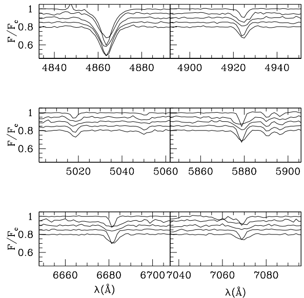
Figure 7. Each panel shows the region of the spectrum where the He features used in this work are located. The spectra are normalized but not red-shifted. In every panel the spectra of the stars A4, A5, A10, A17, A21 are plotted starting from the top and shifted of 0.05 in the y-axis for graphical reasons.
