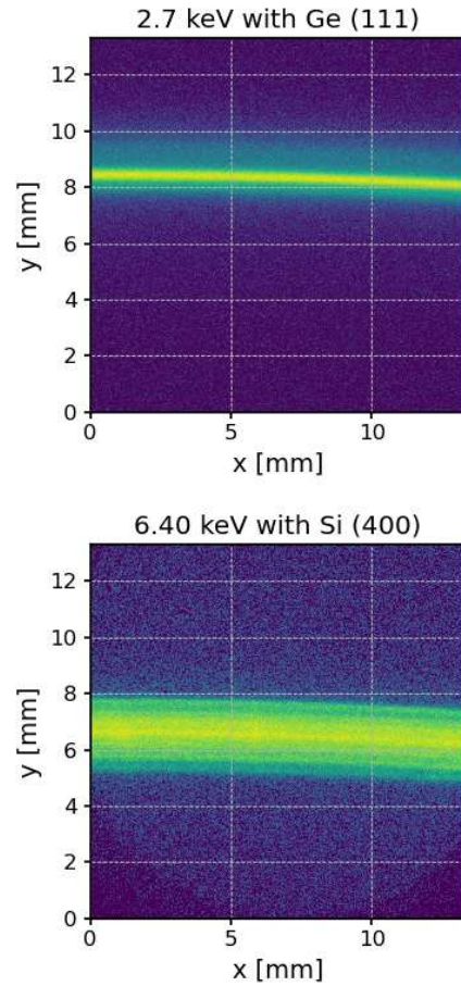
Figure 18: Image with the ICE test imager of the photons generated with the polarized source without collimators. In this condition, diffracted X-rays form a “Bragg” arc on the detector, whose width depends on both the source and the crystal used. On the top there is the Bragg arc obtained with the X-ray tube with Rh anode and the Ge (111) crystal; on the bottom there is the Fe X-ray tube with Si (400) crystal.
