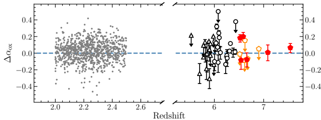
Figure 5. The \Delta\alpha_{\text{ox}} versus redshift plot. All symbols have the same meaning as Figure 4.
