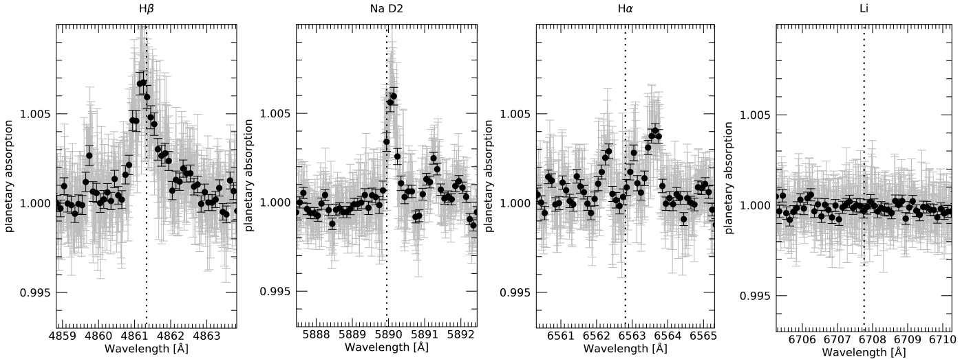
Fig. 13. Transmission spectrum extracted in the zone of the H\beta (left panel), Na D2 (central left panel), H\alpha (central right panel), and Li (right panel) lines. The vertical dashed lines show the planetary restframe. Black points refer to 0.1 Angstrom binning. Different lines we searched for are affected by the contamination given by the stellar activity in different ways.
