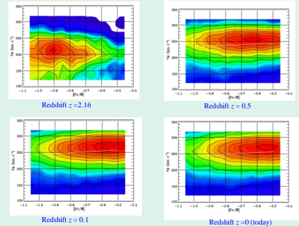
Fig. 5. Distribution V_{\phi} - [\text{Fe}/\text{H}] of the simulated “thick disk” in the “solar” neighborhood, 6 kpc < R < 8 kpc. The white dashed lines show the resulting linear best fit
