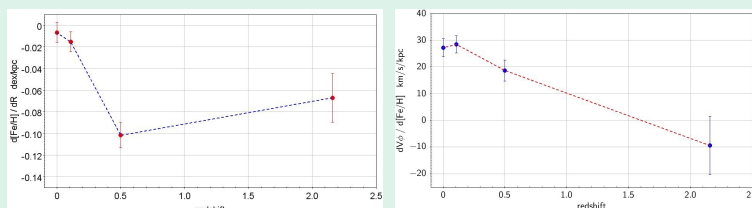
Fig. 6. Evolution of V_{\phi} - [\text{Fe}/\text{H}] and d[\text{Fe}/\text{H}]/dR as a function of time. As in Fig. 5, the values are computed for simulated stellar particles with 6 kpc < R < 8 kpc and 1 kpc < |z| < 3 kpc.
