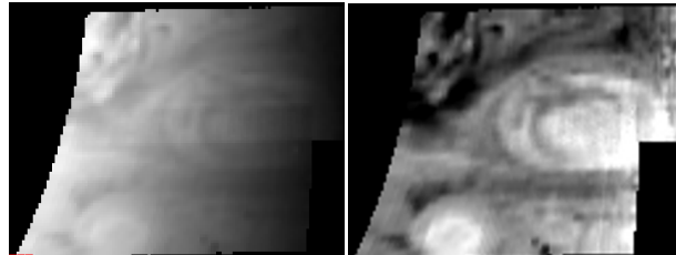
Figure 7 – The Jupiter Great Red Spot, as imaged by NIMS at 2 \mu\text{m} , before (a) and after (b) the Minnaert correction for the viewing and illumination angles.
