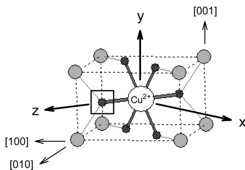
FIG. 4. \text{TiO}_2 (rutile) crystal structure showing a \text{TiO}_6 unit. A \text{Cu}^{2+} ion substitutes for a \text{Ti}^{4+} ion and has an oxygen vacancy along the [110] direction. The x , y , and z directions are the principal-axis directions for the \mathbf{g} , \mathbf{A} , and \mathbf{P} matrices.
