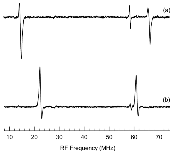
FIG. 6. ENDOR spectra of ^{63}\text{Cu} nuclei in a \text{TiO}_2 (rutile) crystal. These data were taken at 15 K with the magnetic field along the [001] direction. (a) The magnetic field was set at 316.146 mT, which in the ENDOR cavity corresponded to the lowest-field allowed line in the EPR spectrum in Fig. 1. (b) The magnetic field was set at 325.707 mT, corresponding to the highest-field allowed line in the EPR spectrum in Fig. 1.
