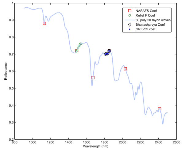
Fig. 3. Hyperspectral signal for 80% Polyester 20% Rayon woven blend with the respective feature set coefficients for the different feature selection methods.
