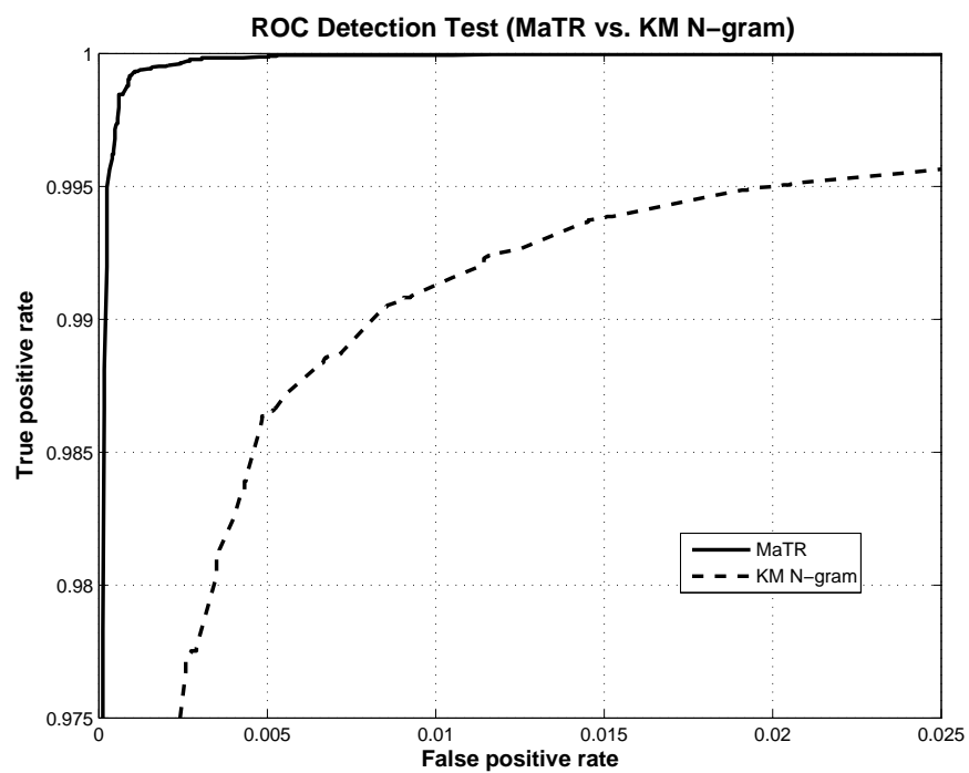
Figure 3: ROC curves for MaTR and KM n -gram retest.
