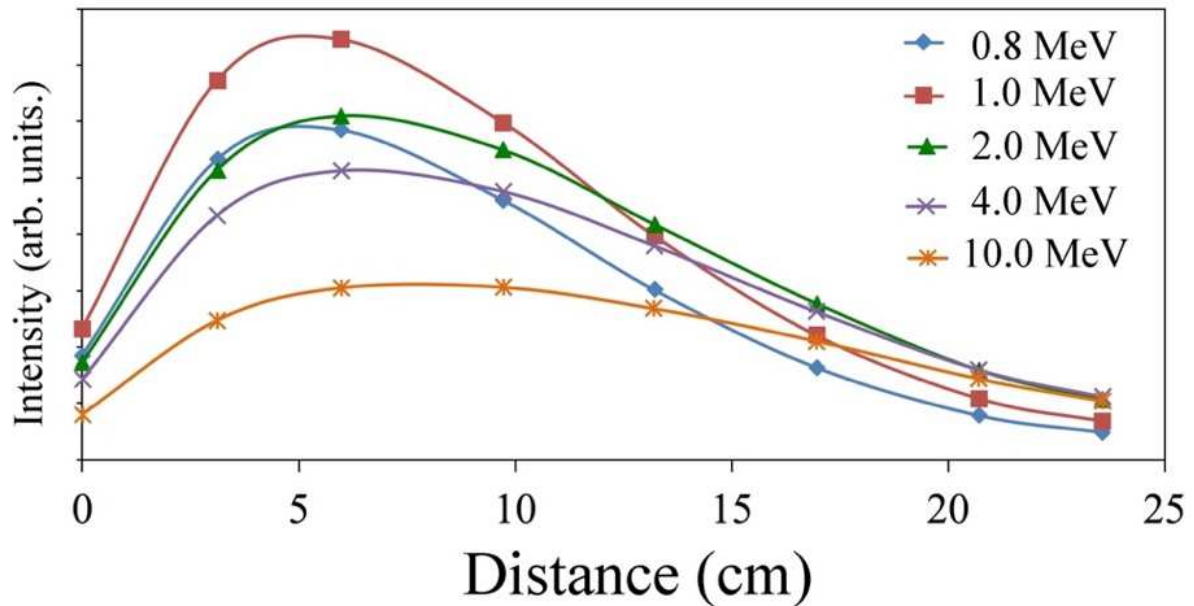
Figure 5. The predicted neutron capture distribution for neutrons of various incident energies, based on MCNP6, as a function of distance into the DANSON detector, taking also into account that the entire detector package is behind approximately 4.6 cm of aluminum and 1.5 cm of steel representing the ISS bulkhead and hatch between the detector package and the outside space environment.
