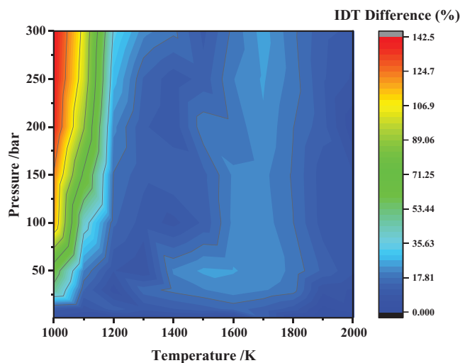
FIGURE 8 Contour plot of the difference in ignition delay time at pressures from 1–300 bar and 1000–2000 K with \text{CH}_3\text{O}_2 chemistry included in the UoS \text{sCO}_2 2.1 mechanism.
