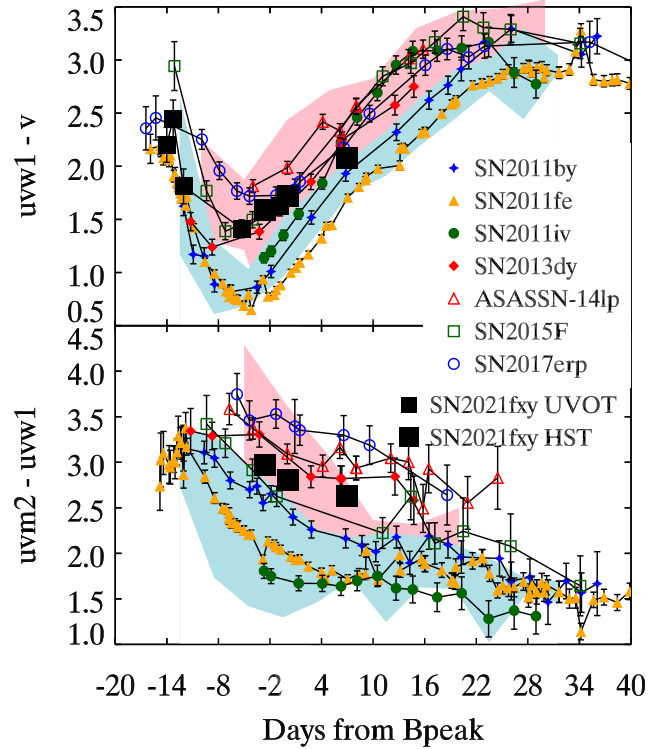
Figure 4. UV colour evolution of SN 2021fxy compared to other spectroscopically normal SNe Ia with HST UV spectroscopy. The pale blue and red polygons note the locations of NUV-blue and NUV-red objects, respectively, as defined in Milne et al. (2013). The larger black squares are synthetic measurements derived from HST /STIS UV spectral observations of SN 2021fxy and the Swift /UVOT filters (Breeveld et al. 2011).
