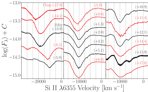
Figure 17. Comparison of Si II \lambda 6355 line evolution in SN 2021fxy and SN 2017erp.
