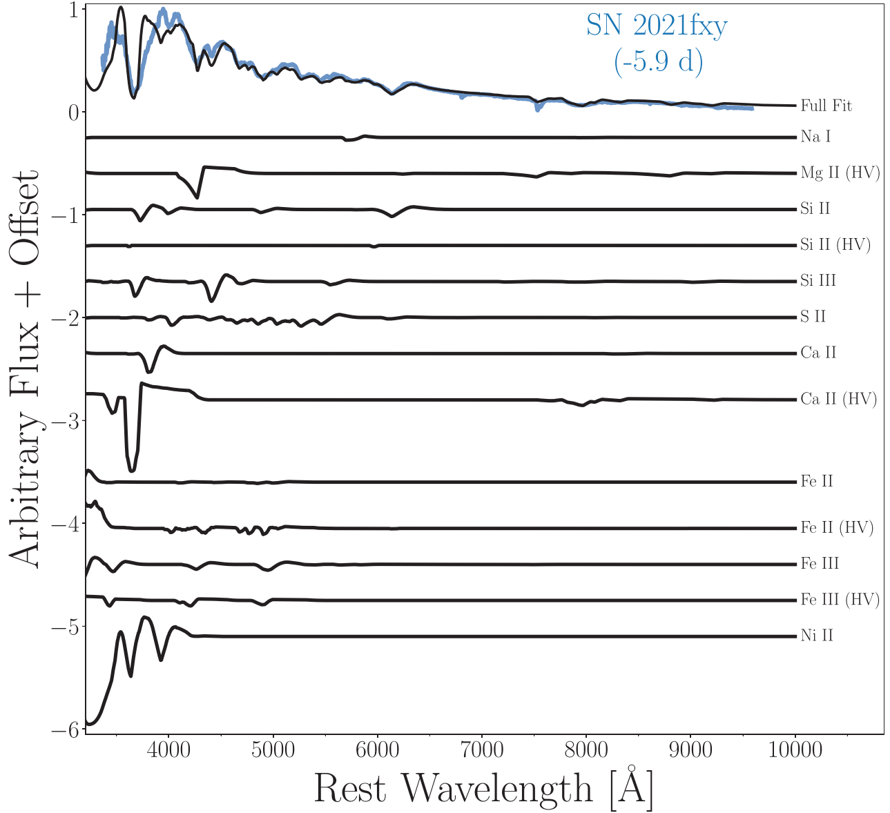
Figure B2. Continuum normalized single-ion fits to the -5.9 -d spectrum of SN 2021fxy (blue), with the complete best fitting model overlaid in black.
