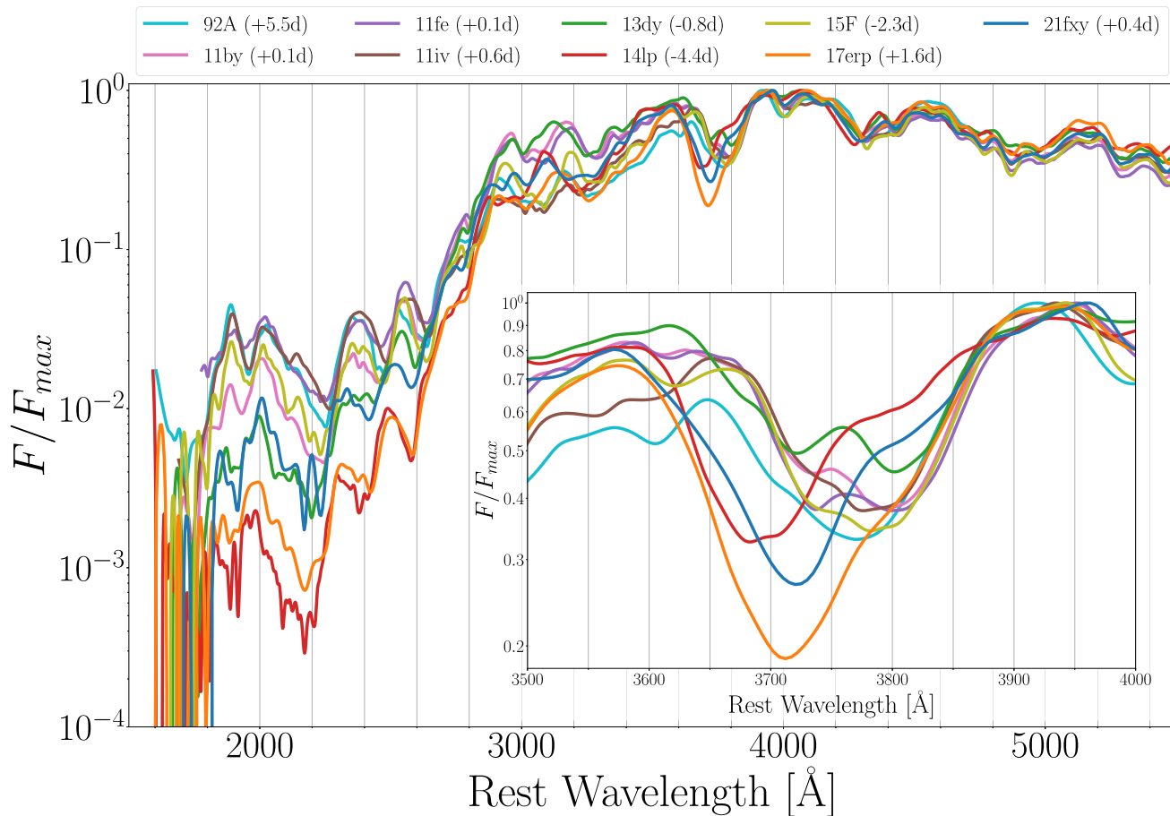
Figure 11. Comparison of SN 2021fxy with other spectroscopically normal SNe Ia having HST /STIS spectra, corrected for Milky Way extinction. Spectra are normalized relative to the maximum flux, which is located at either the Ca II H&K emission peak or the Si II blend emission peak at \sim 4075 Å. Along with SNe 2013dy, ASASSN-14lp, and 2017erp, SN 2021fxy shows suppressed flux in the mid-UV and blue-shifted mid-UV features relative to SNe Ia without suppressed mid-UV fluxes. Inset: Close up of the Ca II H&K features, showing that SNe Ia with MUV flux suppression have strong HV Ca II H&K components which dominate the feature.
