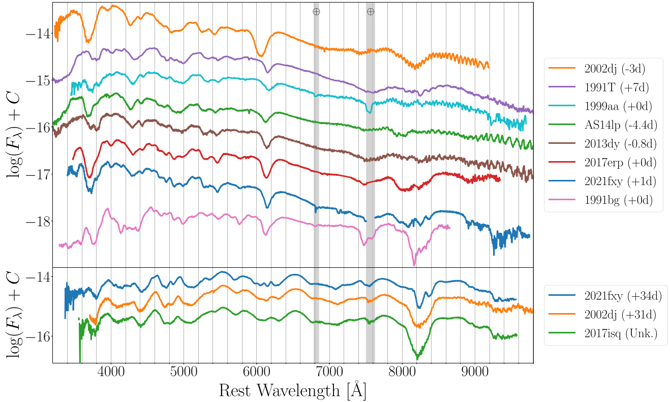
Figure 6. Top Panel: Comparison of SN 2021fxy near maximum light to its sibling SN 2002dj (BL), SN 2017erp (CN), SNe 1991T, 1999aa, 2013dy, and ASASSN-14lp (SS), and SN 1991bg (CL). Bottom Panel: Comparison of siblings SNe 2002dj and 2021fxy to potential sibling SN 2017isq roughly one month after maximum light.
