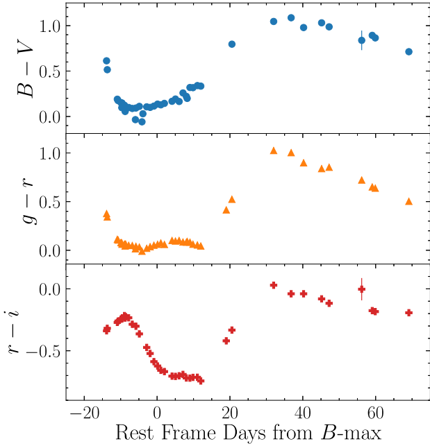
Figure 3. B - V , g - r , and r - i colour curves of SN 2021fxy in the CSP natural system.
