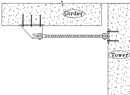
Fig. 5 - Damping Diagram of Elastic Cable
