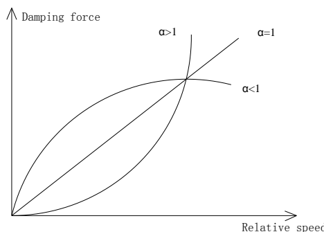
Fig. 2 - Relation between Damping Force and Relative Velocity
