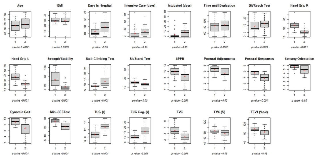
Figure 2 - Box plot of tests by Cluster with indication of means (in red circles) and p-values for the Student's t-test. SPPB, short physical performance battery; BMI, body mass index; D, dominant; ND, no dominant; TUG, Timed Up and Go; TUG-COG, Timed Up and Go Cognitive; FEV1, forced expiratory volume in 1 second; FVC, forced vital capacity.
