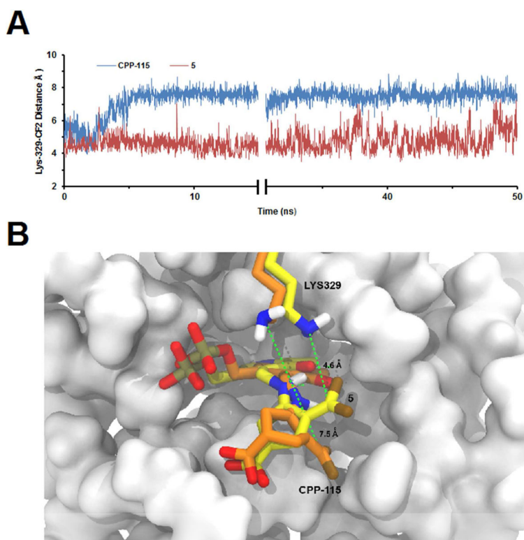
Figure 2. Classical molecular dynamics simulations of CPP-115 and 5 bound to PLP of GABA-AT. Color legend: Yellow or orange-carbon; white-hydrogen; red-oxygen; blue-nitrogen; brown-fluorine; taupe-phosphorus. (A) Distance measurements during the 50 ns of the trajectories between the catalytic Lys329 nitrogen atom and the inhibitors after tautomerization (see Scheme 2). The simulation of CPP-115 's tautomer stabilized after about 4 ns of simulation as a result of a conformational change within the ring, which increased the distance between the CF 2 group and Lys329 to about 7.5Å. This distance with 5 was only 4.6Å (B) Superimposition of the average equilibrated poses of CPP-115 (orange) and 5 (yellow); average distances from the \epsilon -nitrogen of Lys329 to the CF 2 carbon atom are shown, calculated using the last 40 ns of the trajectories.
