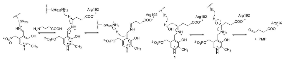
Scheme 1. Catalytic mechanism of GABA-AT for the degradation of GABA into succinic semialdehyde
