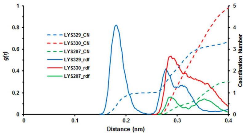
Figure 6. Radial distribution function (rdf) of water around Lys329, Lys330, and Lys207 in the CPP-115 -GABA-AT complex. A well-ordered hydration sphere can be observed around 1.8Å of the terminal nitrogen atom of Lys329, whereas a more disordered one exists for all three lysines between 2.5 and 4Å.
