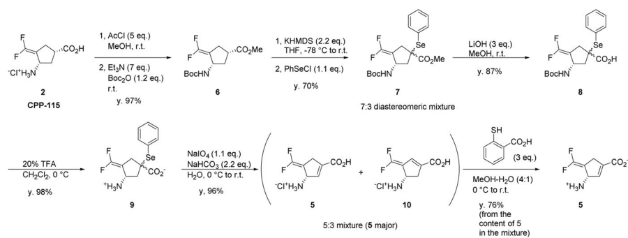
Scheme 3. Synthesis of ( S )-3-amino-4-(difluoromethylenyl)cyclopent-1-ene-1-carboxylic acid ( 5 ) from CPP-115 ( 2 ).
