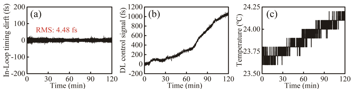
Figure 4. Timing drift measurement of the 200-TW preamplifier over 120 minutes. (a) In-loop timing drift, (b) the DL control signal, and (c) environment temperature fluctuation.
