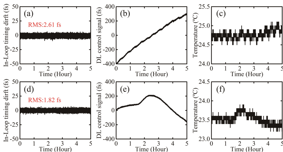
Figure 3. Regenerative amplifier timing drift measurement results without MPC for more than 5 hours (a) in-loop timing drift, (b) the DL control signal, and (c) environment temperature fluctuation. (d)-(f) show the measurement results of the in-loop timing drift, DL control signal, and temperature variation over 5 hours with MPC in the optical path, respectively.
