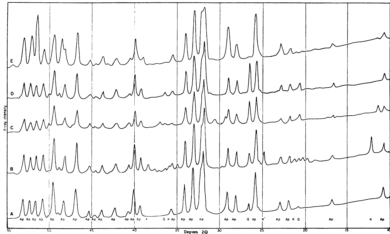
FIG. 1. —Smoothed traced spectrogoniometer record of x-ray scattering distribution. A , 5020, nodules from Muncie Creek shale; B , 52263, nodules from Heebner shale; C , 5021, nodules from Pleasanton shale; D , Bureau of Standards 56b, Tenn. brown rock phosphate; E , crystalline fluoapatite. Abbreviations: Ap, apatite; Q, quartz; and K, kaolin. Records prepared by Ada Swineford using nickel-filtered copper radiation.
