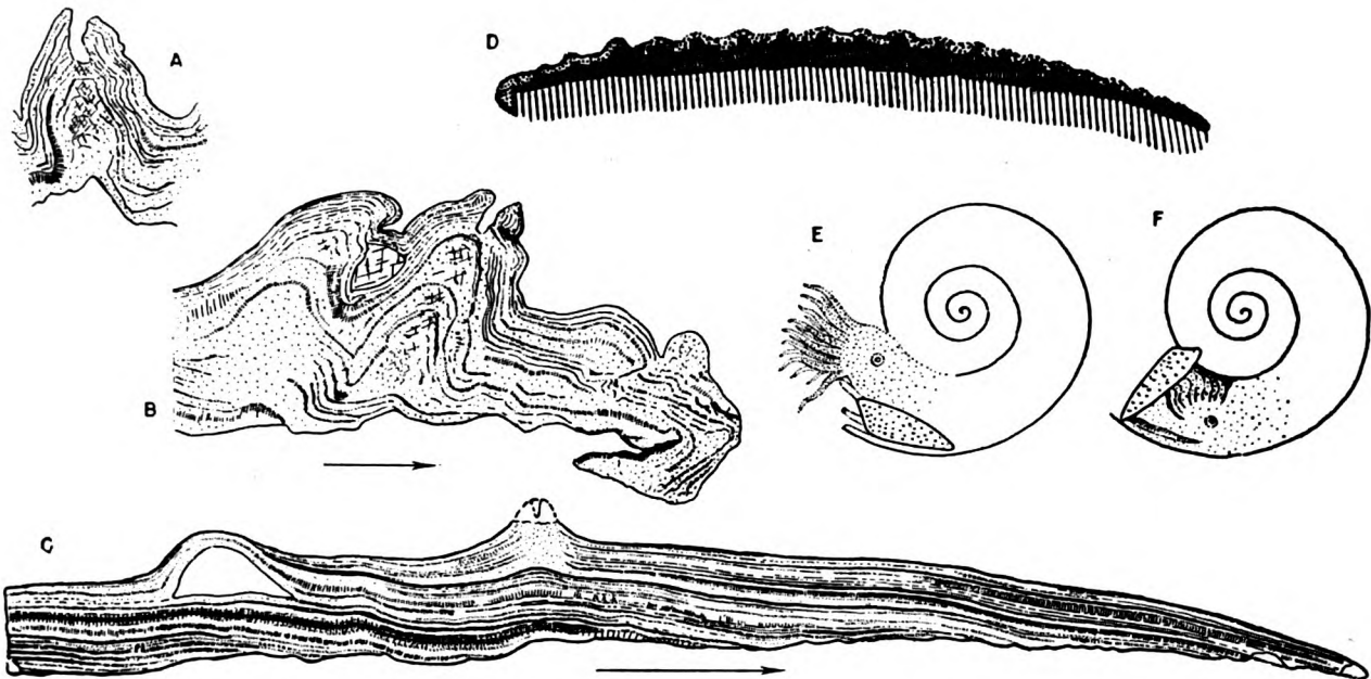
FIG. 1.—Thin sections and restorations of aptychi. Arrows indicate direction toward ventrolateral margin. A, Mus. no. 2684, section across a gerontic aptychus near ventrolateral margin ( \times 15 ). Large tubercle showing canal in upper part and structureless calcite crossed by occasional growth laminae in middle and lower parts. B, Mus. no. 2684, thin section of tubercles of a gerontic aptychus close to ventrolateral margin which in this specimen is curled under ( \times 15 ). C, Mus. no. 2907a, radial section cut to the edge of the ventrolateral margin of an immature specimen. Note imbrication of growth lamellae and cross section of nonperforate blisterlike tubercle ( \times 24 ). D, Diagrammatic dorsoventral section of aptychus and restored tissues. Tissues of attachment are crosshatched, secreting tissue stippled. E, Restoration, head extended. F, Restoration, head withdrawn.
