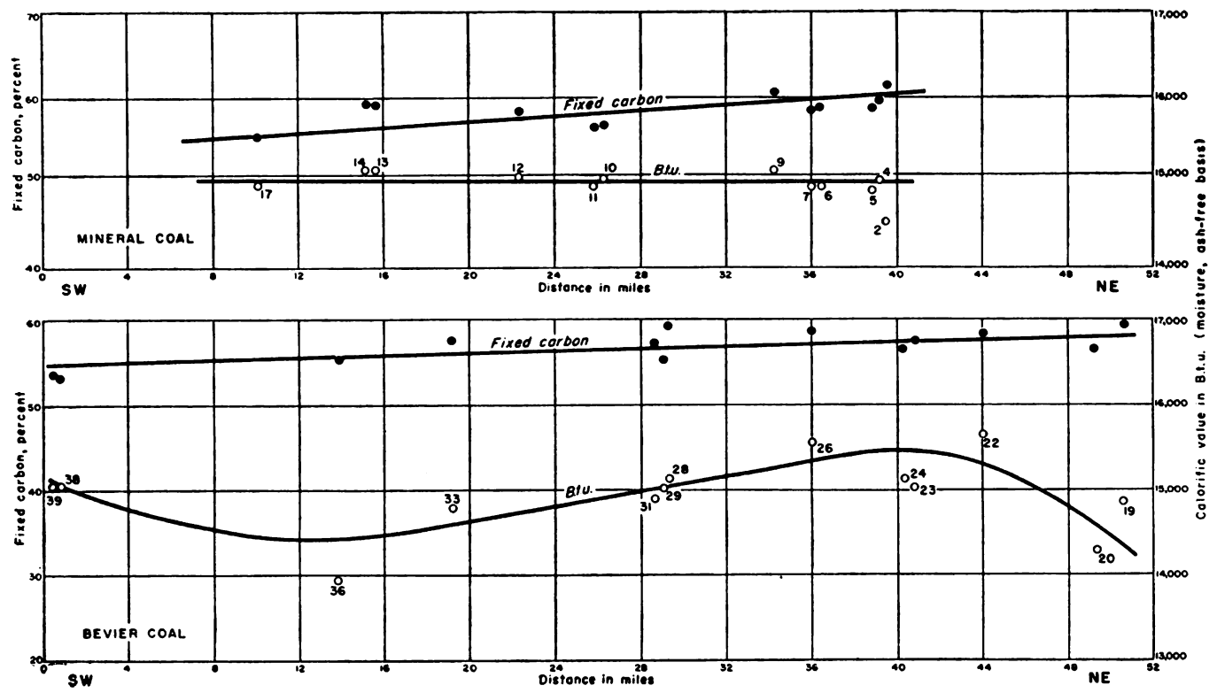
FIG. 4.—Regional variation of fixed carbon and B.t.u. values in Mineral and Bevier coals. (Numbers refer to locations projected to line a-a', Fig. 1.)
