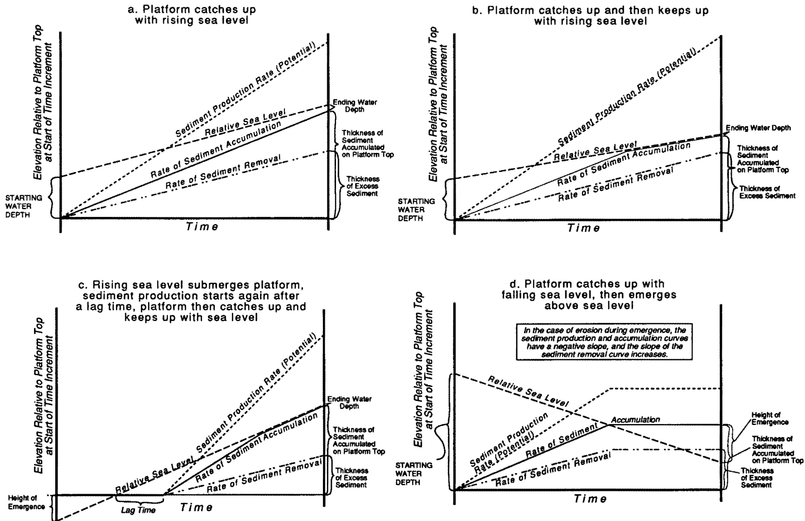
Figure 3. Response of the platform and the generation of the sediment budget under four different conditions. In each diagram the length of time is of the order of 10,000 years so that the relative sea-level curves can be approximated by a straight line. The horizontal line at the base of each diagram is the position of the platform top at the beginning of the time increment. An explanation of these four scenarios is given in the text.
