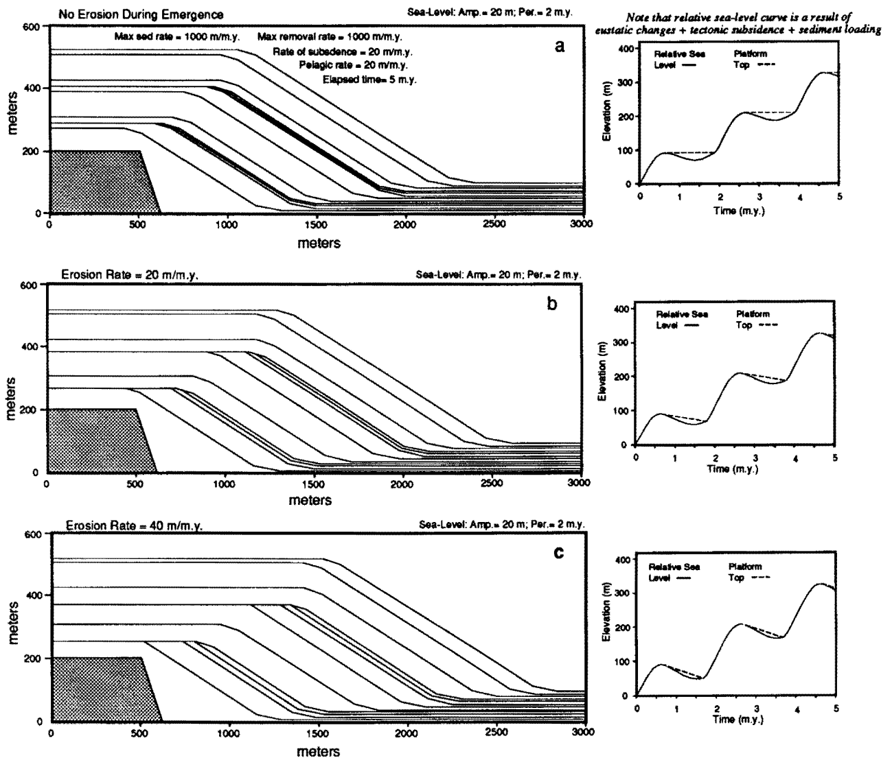
Figure 9. The effect of varying rates of subaerial erosion during emergence. Subaerial erosion during times of emergence leads to the development of tolap relationships and to more asymmetric relative sea-level curves. The relative low rates of erosion and the small horizontal dimension of the platform top combine to minimize the amount of progradation that occurs during times of exposure.
