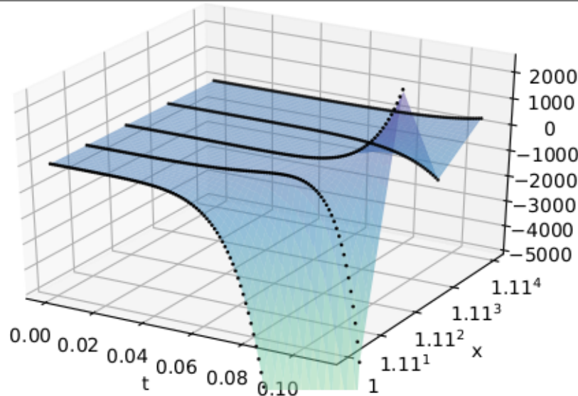
Fig. 2. The q -case with q = 1.11 and h = 0.001 . The black lines use (4.6) to approximate a solution of (1.1) at each x \in \mathbb{T} for 0 \leq t \leq 0.1 . The initial data is a function g: \mathbb{T} \rightarrow [-0.3, 0.3] whose values were randomly sampled from the uniform distribution on that interval. The colored regions between them is a surface made of linear interpolations to help visualize the structure of the solution
