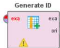
Gambar 4. Generate ID
