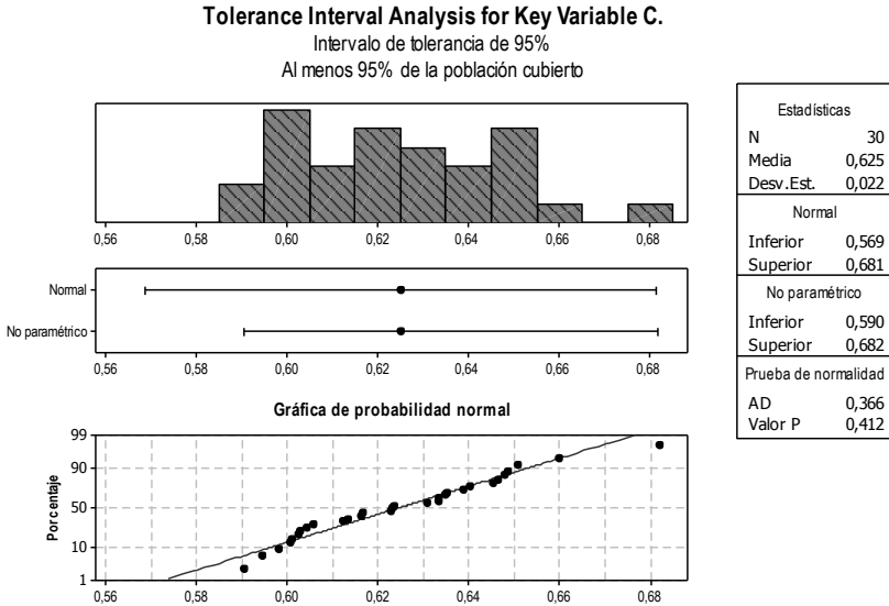
Figure 14. Tolerance Analysis for Key Dimension C (Based on CTQ condition, by Cruz, J.).
