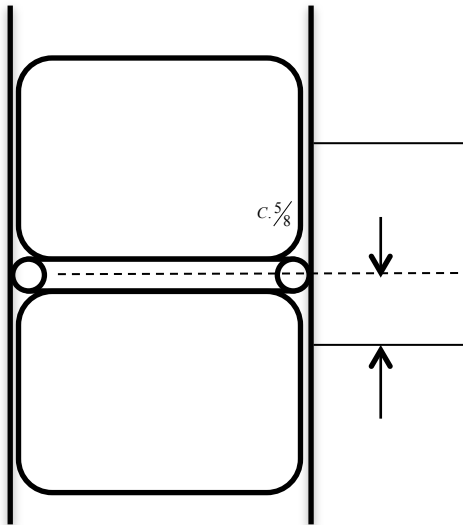
Figure 10. Spout Tube and O`ring Leak Free Feature (by Cruz, J.)
