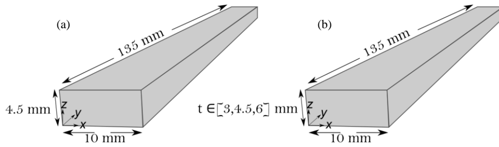
Fig. 12 (a) FDM printed solid beam used for convergence study, (b) infill beams considered for material characterization
