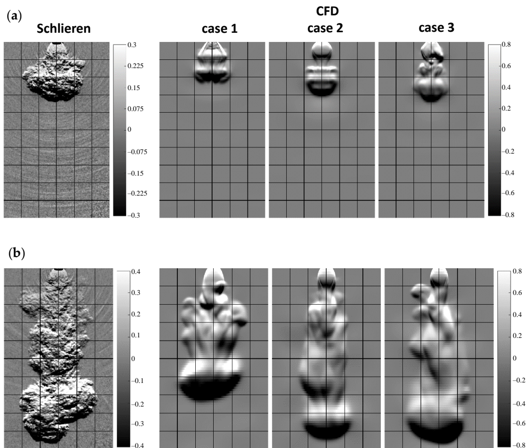
Figure 8. Comparison between Schlieren contrast and numerical results: t = 400 \mu\text{s} (a); t = 975 \mu\text{s} (b).
