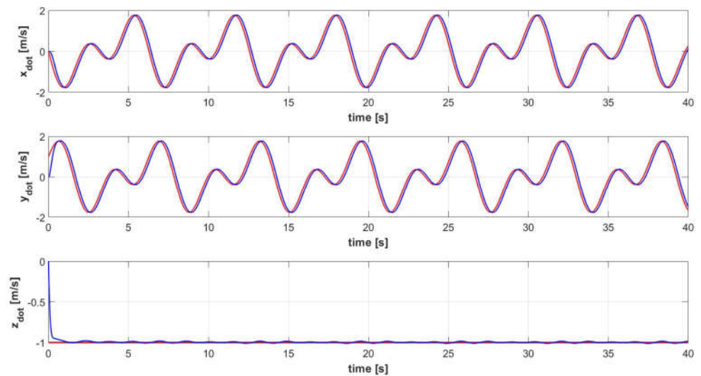
Figure 13. Velocity signals [\dot{X}(t), \dot{Y}(t), \dot{Z}(t)] of the controlled quadrotor system (blue) and reference velocity signals of trajectory 2 (red).
