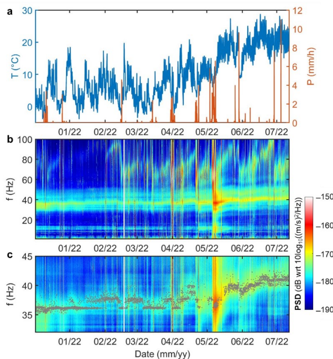
Figure 9. (a) Available meteorological data during the monitored period (ARPA Piemonte): hourly air temperature ( T ) from Pamparato station and precipitation ( P ) from Frabosa Soprana station. (b) Hourly Power Spectral Densities of the N components of Station S1. (c) Zoom of (b) in the frequency band 32–45 Hz. The automatically extracted frequency peaks are overlain with gray dots.
