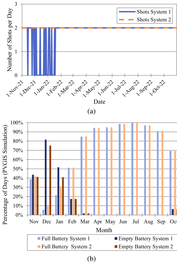
Figure 9. Actual and simulated performances of the system over a year. (a) Number of shots per day of the two systems. (b) Percentage of days in a month when the battery became full or empty according to PVGIS simulations at the location of the two monitoring systems.
