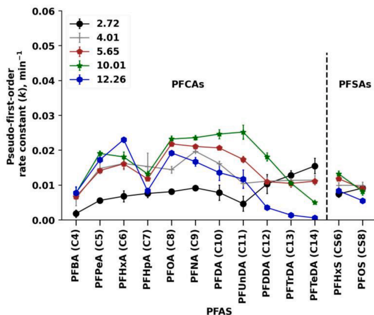
Fig. 4. Pseudo-first-order rate constant ( k ) of perfluoroalkyl carboxylic acid (C4-C14) and perfluoroalkyl sulphonics acid (CS6, CS8) degradation over a range of pH (2.72 – 12.26) at 575 kHz frequency.
