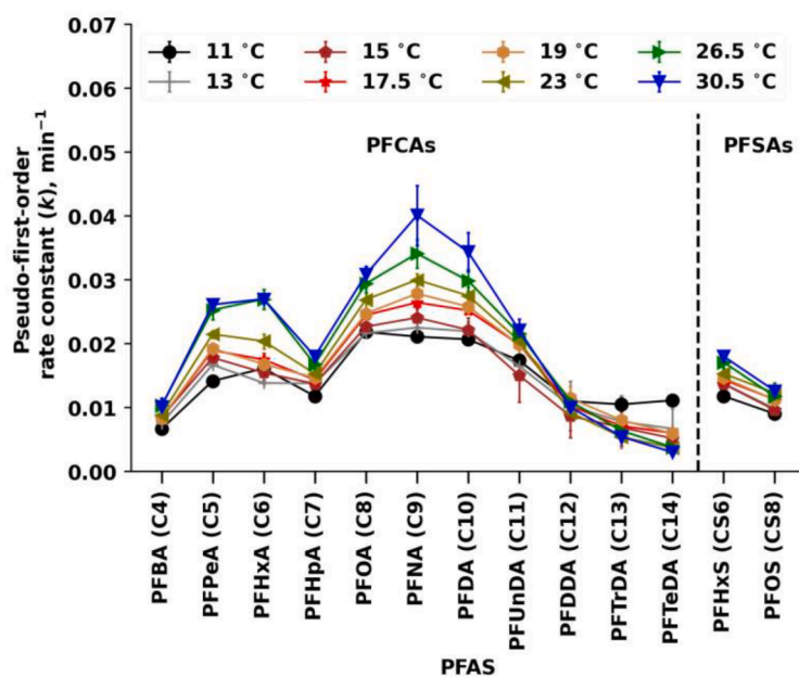
Fig. 5. Pseudo-first-order rate constant ( k ) of perfluoroalkyl carboxylic acid (C4-C14) and perfluoroalkyl sulphonics acid (CS6, CS8) degradation over a range of Temperature (11 – 30.5 °C) at 575 kHz frequency.
