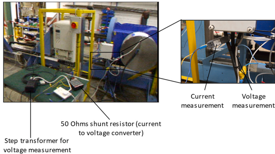
Fig. 6. The experimental system for measuring the current and voltage.
