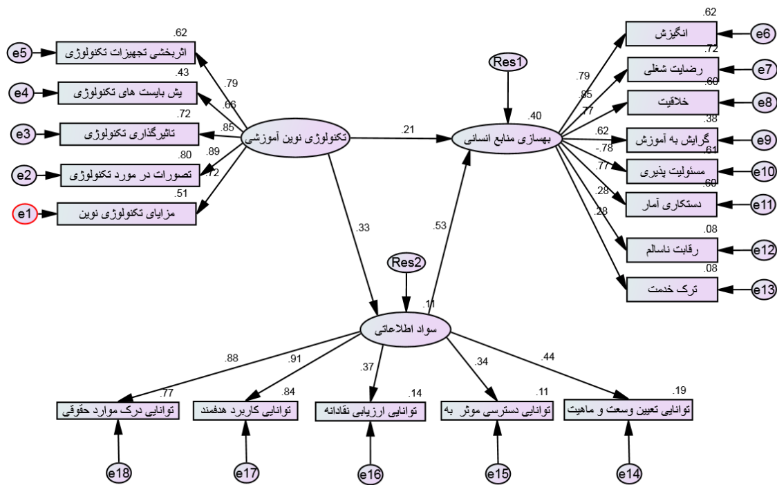
Figure 4. Structural Model in Standard Coefficient Estimation Mode
