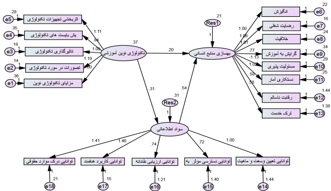
Figure 3. Structural Model in Non-standard Coefficient Estimation Mode
