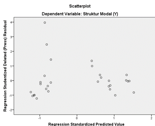
Figure 2. Heteroscedasticity Test
