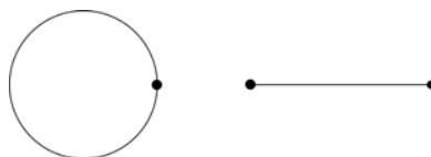
Figure 5: Flat representation of the circle.
