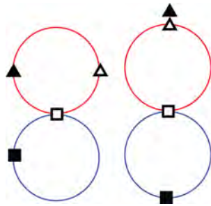
Figure 43: Initial and final positions and their corresponding skeleton positions.
