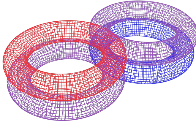
Figure 3: Cartesian product (S^1 \vee S^1) \times (S^1 \vee S^1) .
