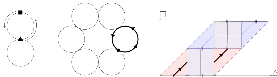
Figure 36: A neighborhood of a vertex position.
