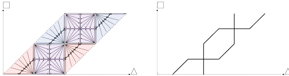
Figure 11: Homotopy traces of the retraction of X into Z .
