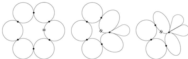
Figure 17: First stages of the deformation.
