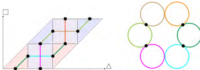
Figure 26: Intersection points in Z and C .
