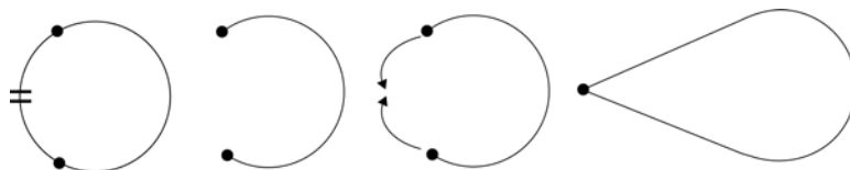
Figure 16: Contraction of a segment in a circle.
