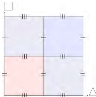
Figure 6: The product \Gamma \times \Gamma
