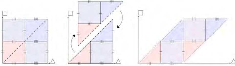
Figure 8: Transition from square to parallelogram representation.
