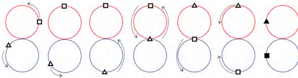
Figure 42: Steps of the algorithm in \Gamma for case 2.
