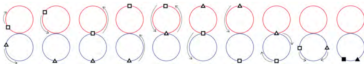
Figure 39: Steps of the algorithm in \Gamma for case 1.
