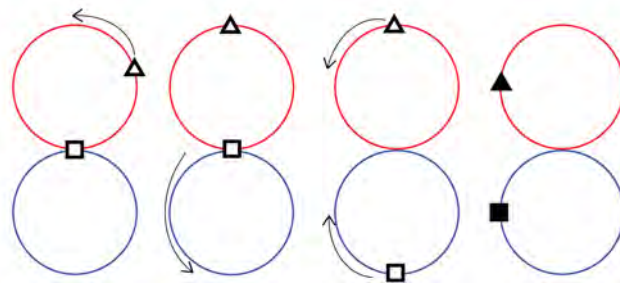
Figure 45: Steps of the algorithm in \Gamma for case 3.
