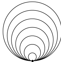
Figure 19: Wedge of seven circles Y .
