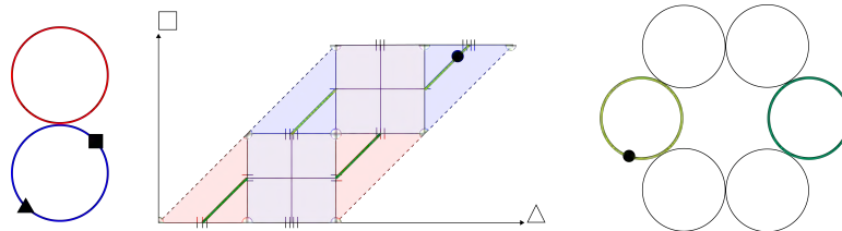
Figure 21: A sub-diagonal state.
