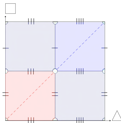
Figure 7: Flat representation of X = (\Gamma \times \Gamma) - D
