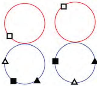
Figure 37: Initial and final positions and their corresponding spine positions.
