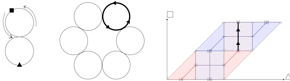
Figure 35: A neighborhood of a non-vertex position.
