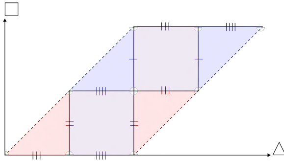
Figure 9: Flat representation of X = (\Gamma \times \Gamma) - D as a parallelogram.
