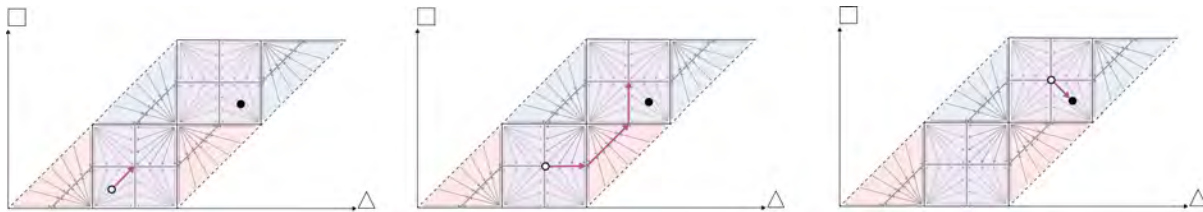
Figure 41: Path in X for case 2.
