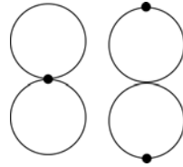
Figure 10: The center and the poles, respectively.
