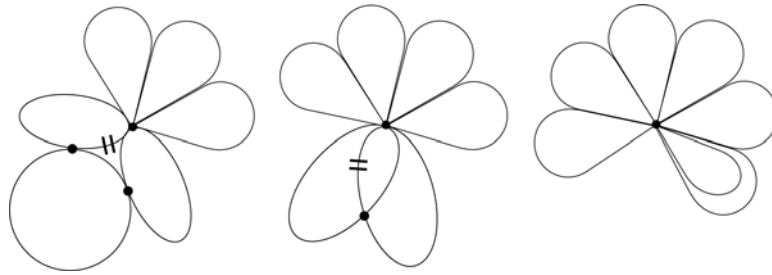
Figure 18: Last stages of the deformation.
