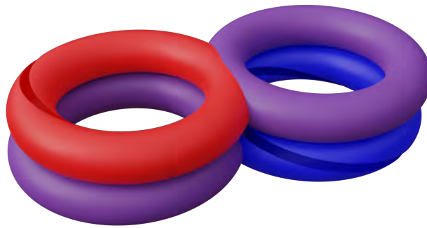
Figure 4: X = (\Gamma \times \Gamma) - D .
