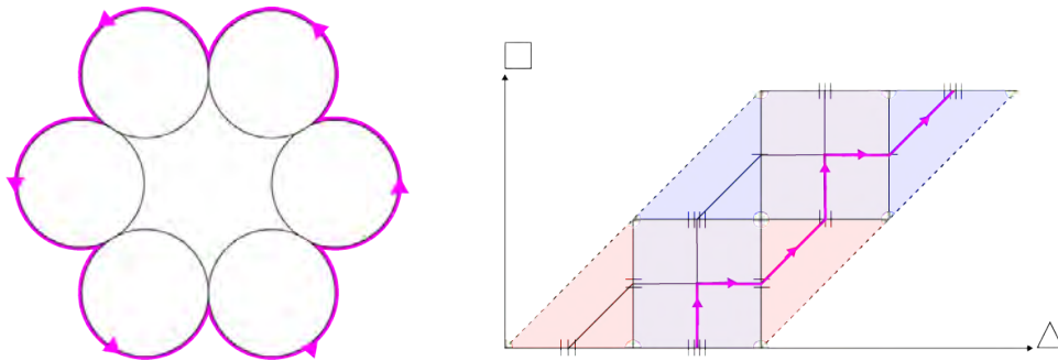
Figure 27: Positive direction in C and Z .
