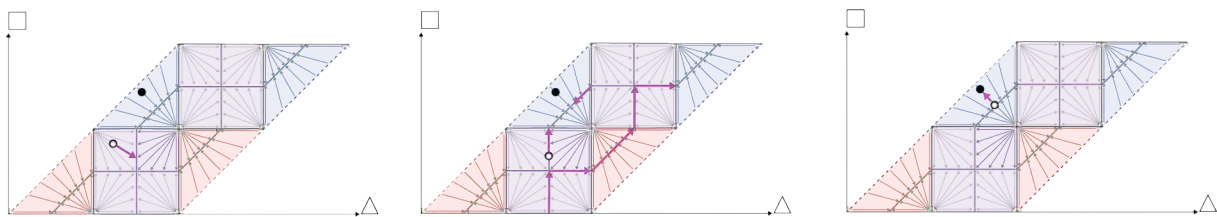
Figure 38: Path in X for case 1.
