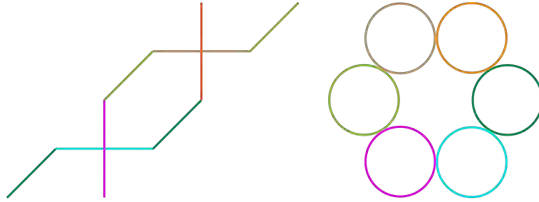
Figure 13: The spine Z is homeomorphic to the chain C .
