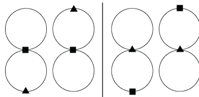
Figure 25: Intersection V-points (left) and H-points (right) in the physical space \Gamma .
