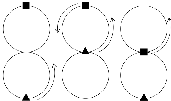
Figure 34: Positive direction in \Gamma .
