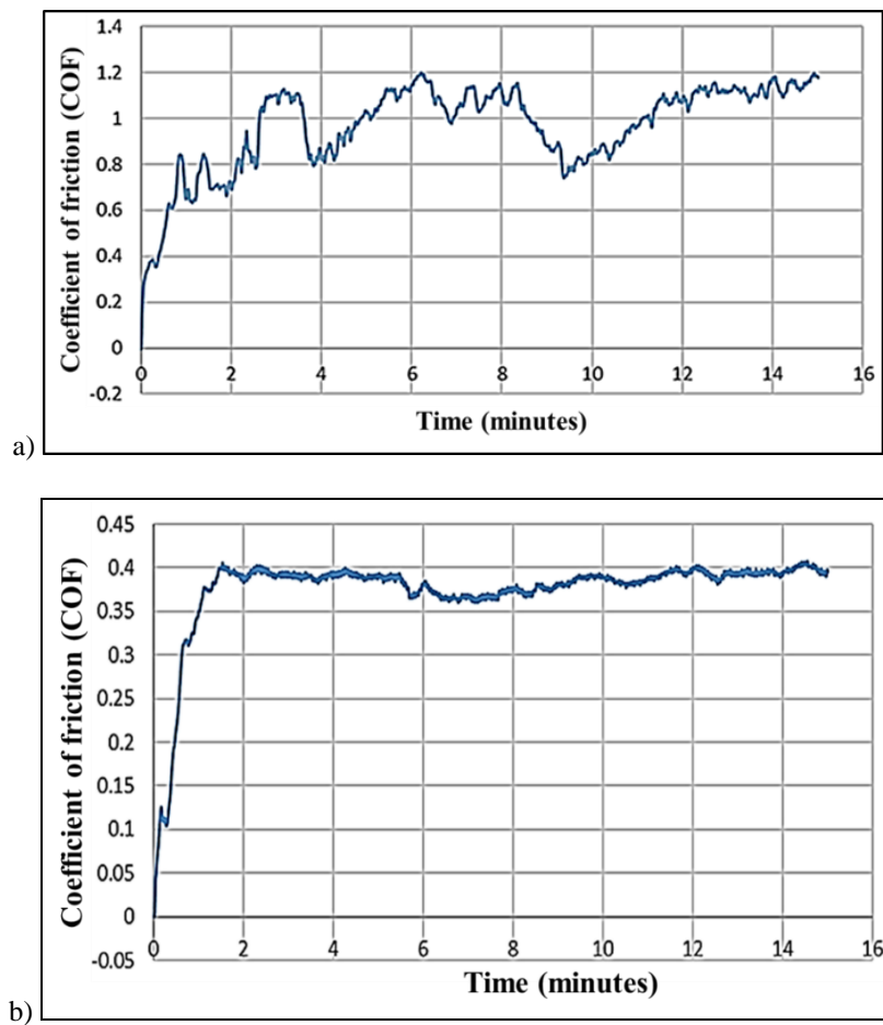
Fig. 9 Variation of COF with time during wear testing of wire-EDM manufactured miniature ratchet gears: (a) poor surface quality miniature ratchet gear; (b) optimized miniature ratchet gear
