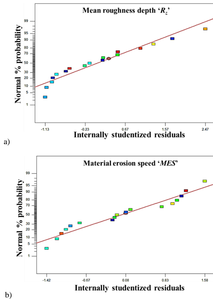
Fig. 4 Normal probability distribution graphs of residuals for selected responses: (a) mean roughness depth ' R_z ' and (b) material erosion speed ' MES '
