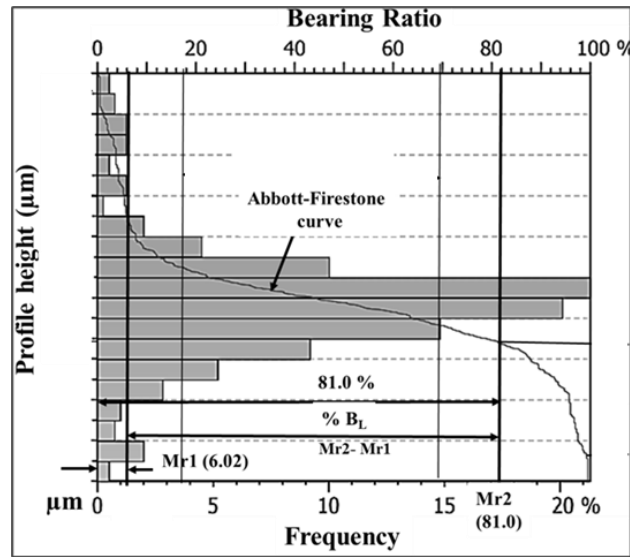
Fig. 7 Bearing area curve for the best surface quality ratchet gear
