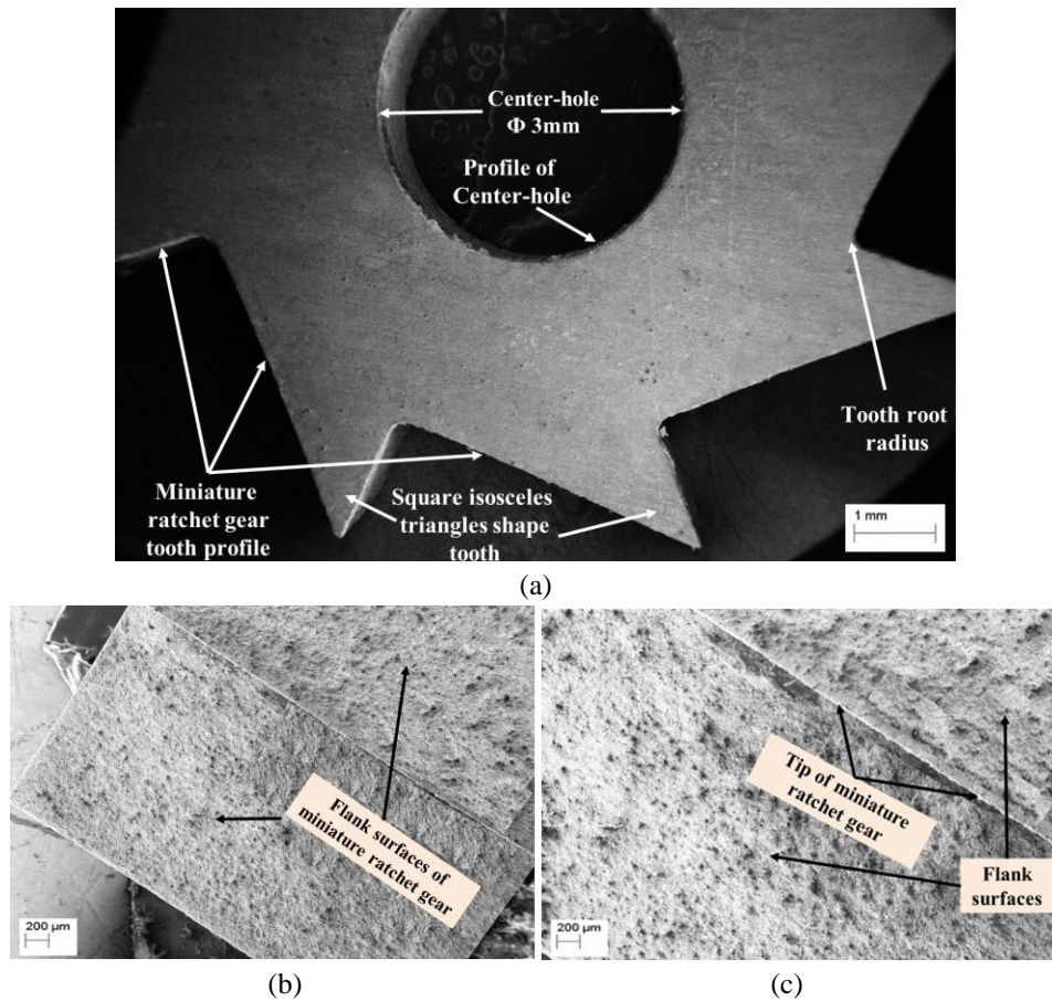
Fig. 10 Scanning electron micrographs of miniature ratchet gear manufactured at optimal parameters of wire-EDM: (a) gear teeth profile; (b) and (c) magnified flank surfaces
