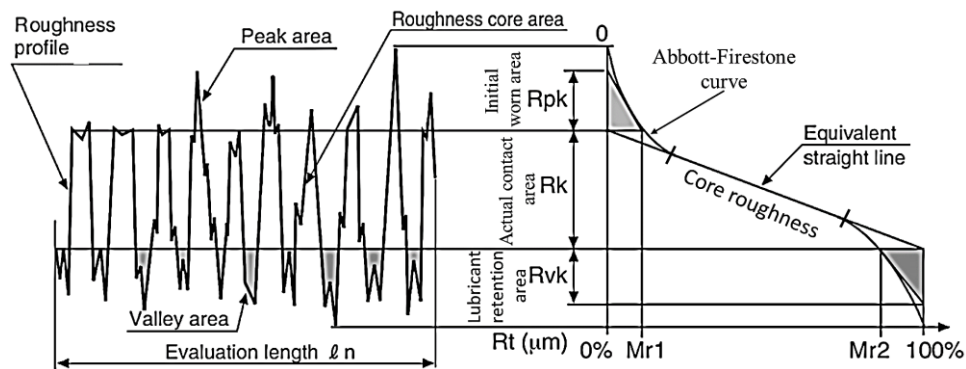
Fig. 6 Theoretical concept of bearing area curve
