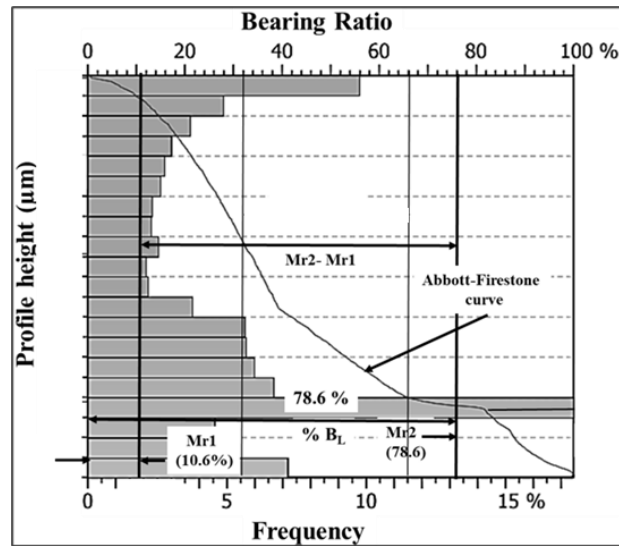
Fig. 8 Bearing area curve for poor surface quality ratchet gear
