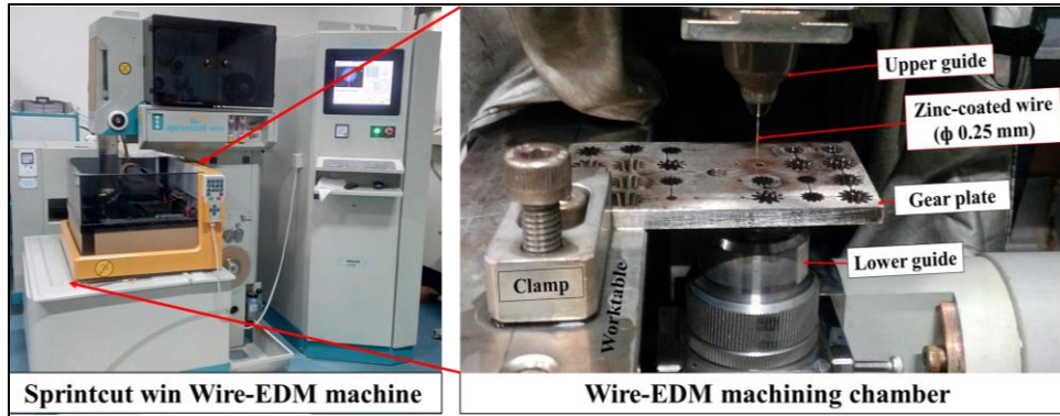
Fig. 2 Wire-EDM machine tool used for this study and enlarged view of machining chamber during cutting of miniature ratchet gear
