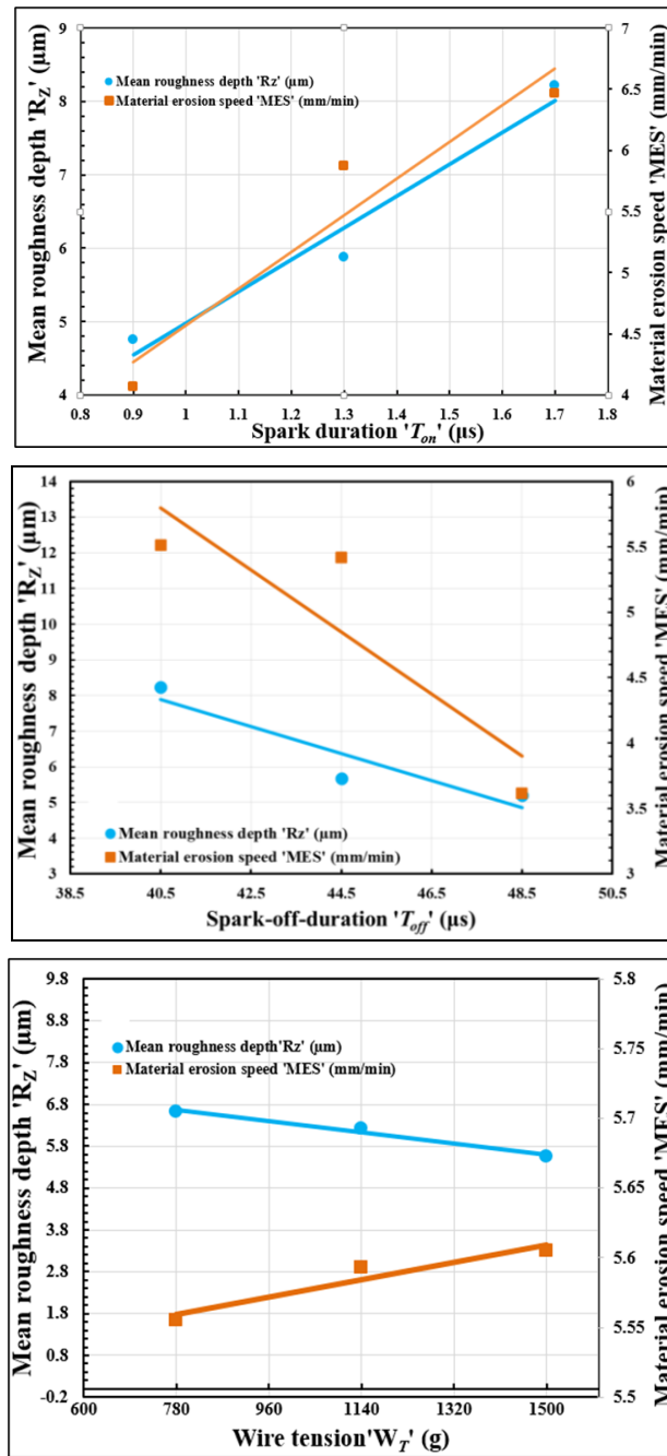
Fig. 3 Effect of wire-EDM parameters on mean roughness depth and material erosion speed during manufacturing of ratchet gear: a) Effect of spark duration; b) Effect of spark-off duration; c) Effect of wire tension
