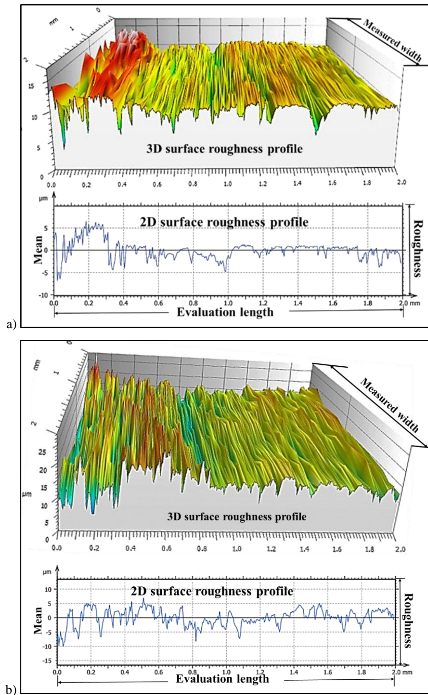
Fig. 5 2D profiles and 3D topographies for surface roughness of (a) best quality ratchet gear, (b) poor quality ratchet gear
