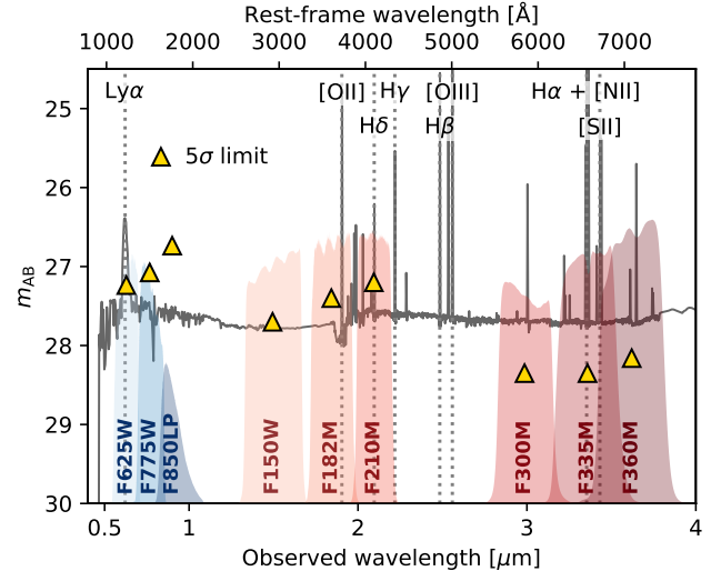
Figure 1. Wavelength range and limiting sensitivities of the photometric observations used in this analysis. Triangles illustrate the 5\sigma limiting magnitudes for the HST/ACS (Zirm et al. 2005) and JWST/NIRCcam (Windhorst et al. 2022) bands, with the corresponding filter transmission profiles shown as blue and red shaded regions respectively. Also shown for reference is a canonical stellar population as seen at z = 4.11 (100 Myr old continuous star-formation history, solar metallicity and zero dust attenuation) with a total stellar mass of 10^8 M_{\odot} . Vertical dotted lines illustrate key UV and optical emission lines, with individual species (or pairs) labelled.
