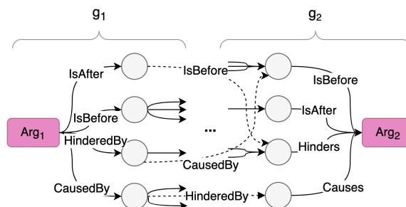
Figure 2: Knowledge graph generation by ARGCON with link inference enabled. The figure shows how two graphs, g_1 and g_2 , are generated from each AU, Arg_1 & Arg_2 , and then merged. Dashed lines show additional relations found by LINK.
