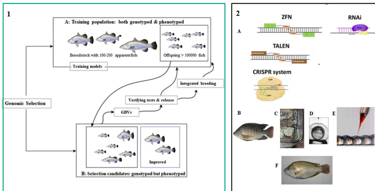
Fig. 2. Genomic selection (GS) and genome editing (GE) enable to rapidly improve economic traits of aquaculture species. 1. Genomic selection. (1-A): The training population is the population, which is phenotyped and genotyped. The broodstock with 100–200 parents used to produce the offspring by crossing selected parents. Offspring are used as a validation set to train the model against the training sets in the training population. (1-B): Selection candidates in breeding populations are only genotyped but not phenotyped. The breeding candidates with highest genomic estimated breeding values (GEBVs) are selected and will be used to produce next generation. 2. Genome editing (GE). There are basically four different approaches for GE, including ZFN, RNAi, TALEN and Crispr/Cas-9. (A). In fish, GE is conducted by microinjection of gRNA and Cas protein into single-cell fertilized eggs. (B): Original fish; C & D: Single cell eggs, E: microinjection and F: gene-edited fish.
