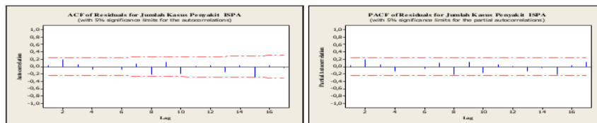
Gambar 4. Plot ACF dan PACF Residual Model ARMA(1,2) Kasus ISPA
