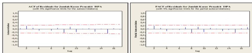
Gambar 5. Plot ACF dan PACF Residual Model ARMA(2,2) Kasus ISPA
