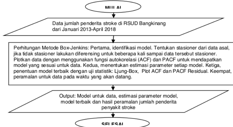
Gambar 1. Flowchart Metodologi Penelitian
