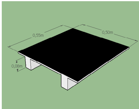
Figure 6 Pallet design paving block (see online version for colours)
