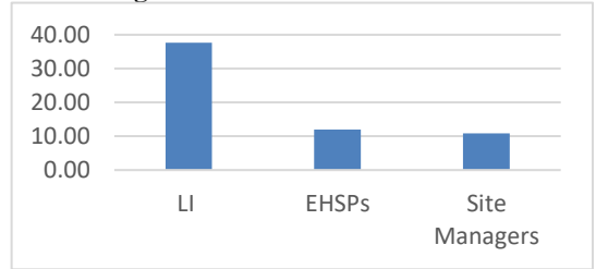
Fig 1. Mean N hazards observed
