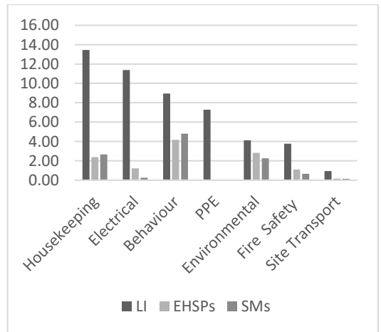
Fig. 2 Mean N hazards observed by construct
