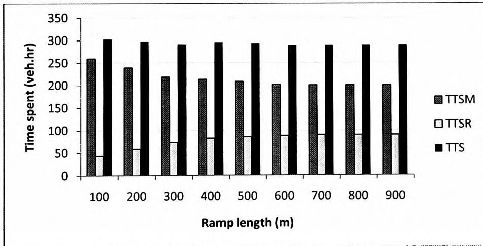
Figure 8-27 Effect of ramp length on the time spent using the ALINEA algorithm
