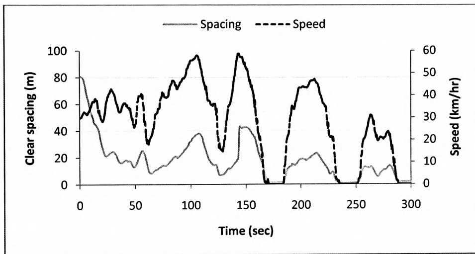
Figure 6-4 Instrumented data Set 1 (from Germany) showing clear spacing and leading vehicle speed profiles based on Panwai and Dia (2005)
