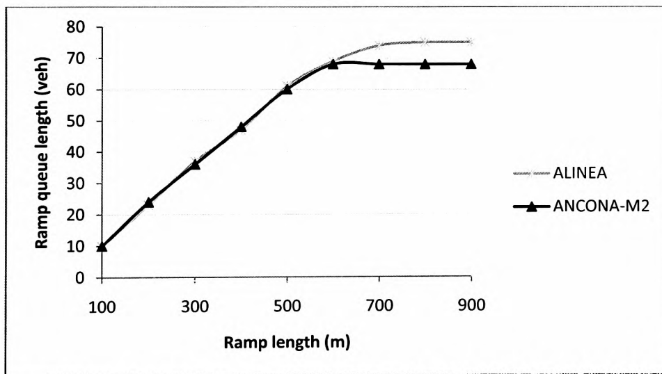
Figure 8-31 Comparison between queue lengths obtained by using the ALINEA and ANCONA-M2 algorithms
