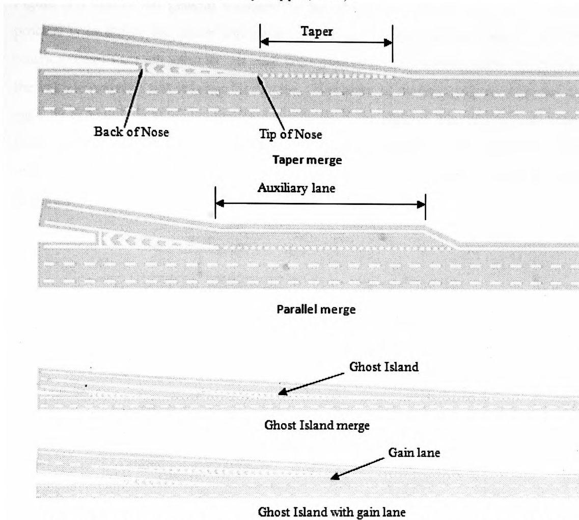
Figure 5-1 Geometric layout considered in the model (Highways Agency, 2008)
