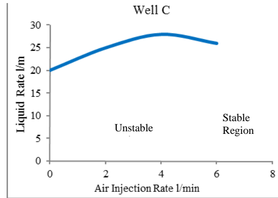
Fig. 10 Effect of injection rate on well performance
