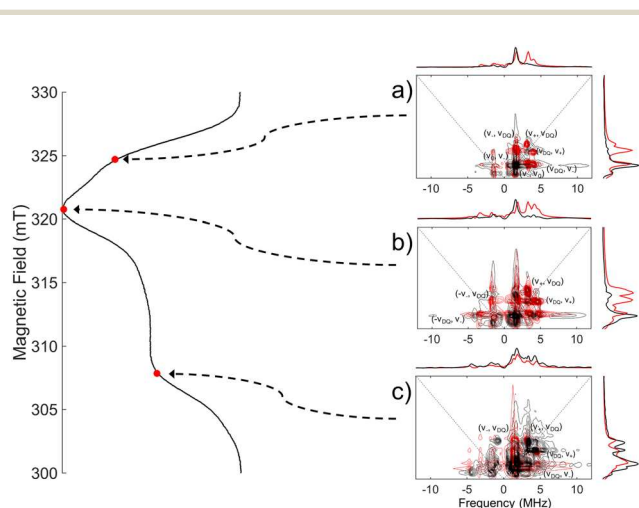
Fig. 6 Simulation (in red) of the X-band ^{14}\text{N} HYSCORE spectrum (in black) of Ni II –NO adduct in Ni-MFU-4l-NO 2 recorded at (a) 325.0 mT, (b) 320.8 mT, and (c) 309.0 mT. The ESE detected EPR signal of Ni II –NO is reported on the left side. Spectra were recorded at 10 K.
