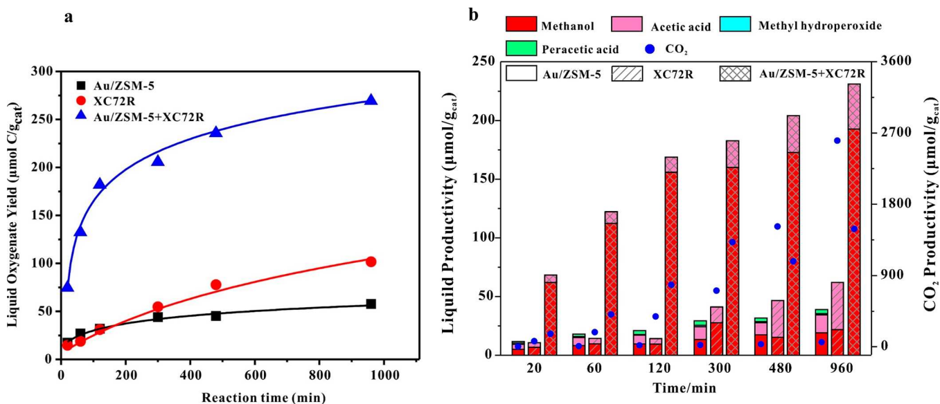
Figure 2. Promotional effect of XC72R addition on the catalytic performance of Au/ZSM-5, as a function of reaction time (a) total oxygenate yield, (b) liquid oxygenate and CO 2 productivity. Reaction conditions: Au/ZSM-5 (0.1 g), XC72R (0.08 g), H 2 O (15 mL), 240 °C, CH 4 (20.7 bar), O 2 (3.5 bar), 1000 rpm.
