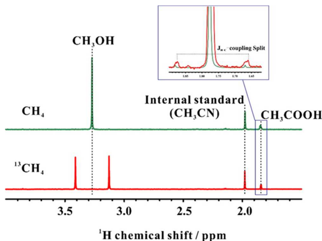
Figure 3. ^1\text{H} NMR spectra of the products obtained from the reactions using \text{CH}_4 in natural abundance or ^{13}\text{C} -labeled ^{13}\text{CH}_4 as reactant. Insertion: Enlarged and normalized J_{\text{H-C}} -coupling region of the methyl group of acetic acid.
