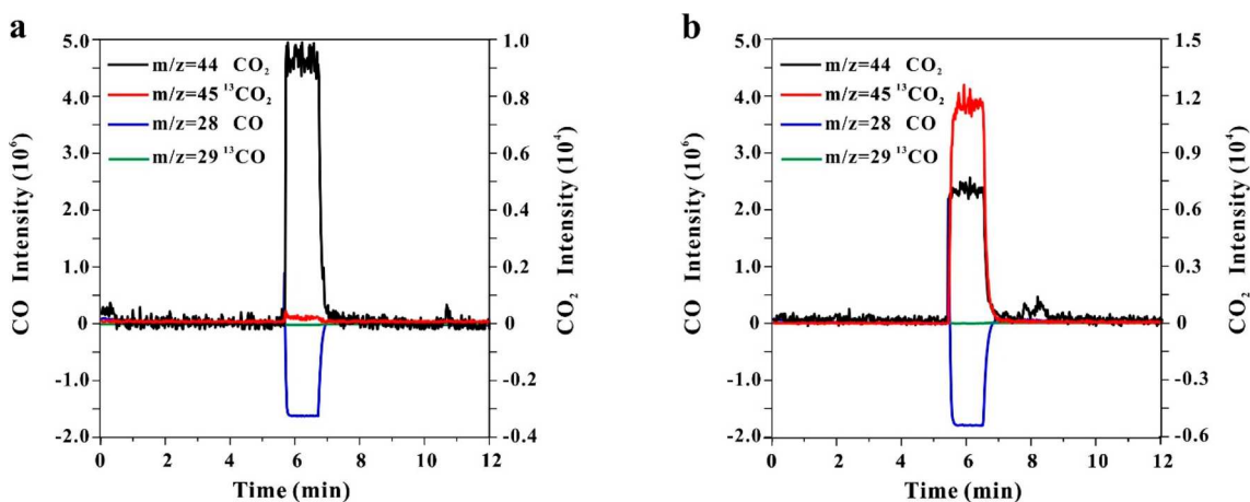
Figure 4. Mass spectrometry analysis of gas products obtained from the reactions using (a) ^{12}\text{CH}_4 and (b) ^{13}\text{CH}_4 as reactant.
