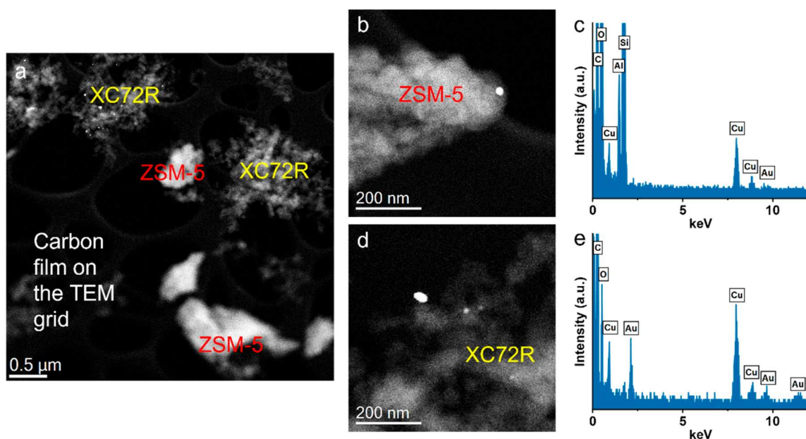
Figure 1. AC-STEM characterization of the Au/ZSM-5 and XC72R (0.08 g) catalyst after the methane oxidation reaction. (a) A lower magnification HAADF-STEM image, showing XC72R particles and ZSM-5 particles in the same field of view. (b, c) HAADF images and the corresponding X-ray energy dispersive spectrum of (b, c) a ZSM-5 particle and (d, e) a XC72R particle.
