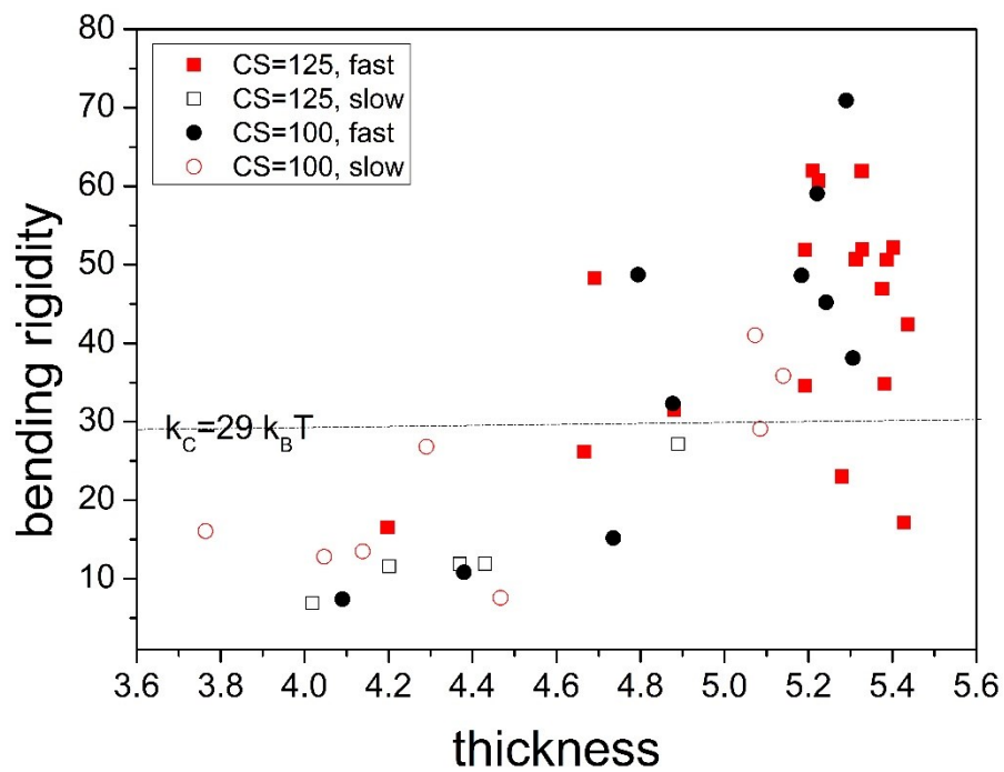
Figure S4 The relationship between vesicle membrane thickness and bending rigidity.
