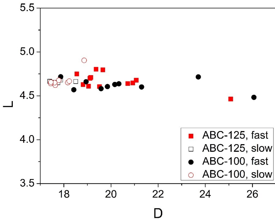
Figure S3 The relationship between membrane diameter and thickness.
