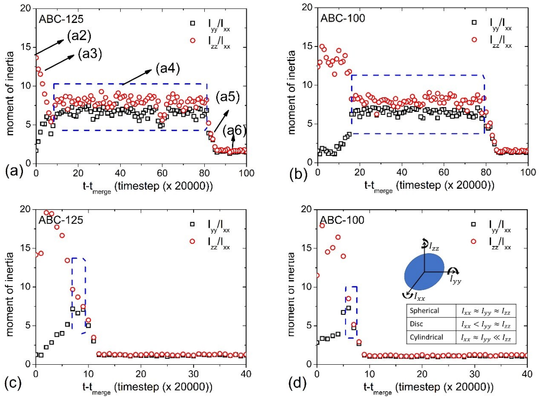
Figure S2 Evolution of geometry of aggregates monitored by their moment of inertia with narrow time span.
