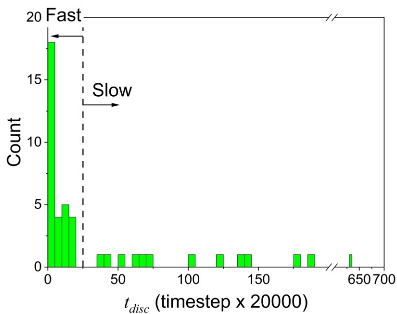
Figure S1 The distribution of lifetime of disk micelles.
