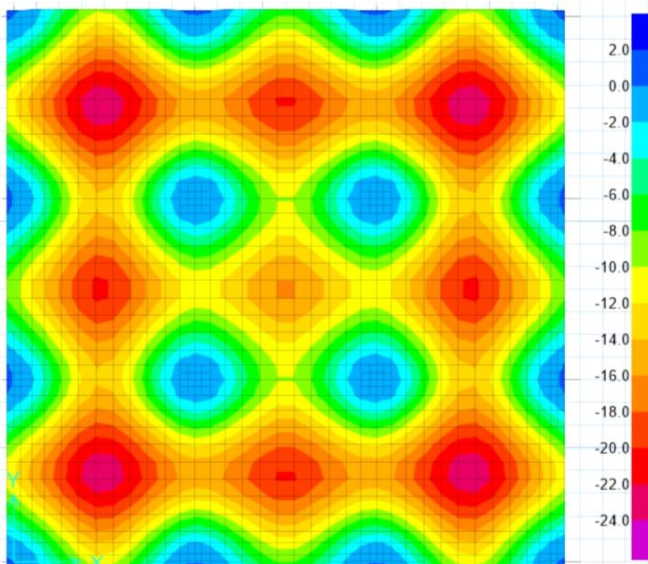
Figure 6. Long-term deflection for flat slab with drop (L=4m, LL=4.5 kN/m 2 , f'_c = 21\text{MPa} , t=290 mm and t_2=0.25t_{\text{slab}} )
