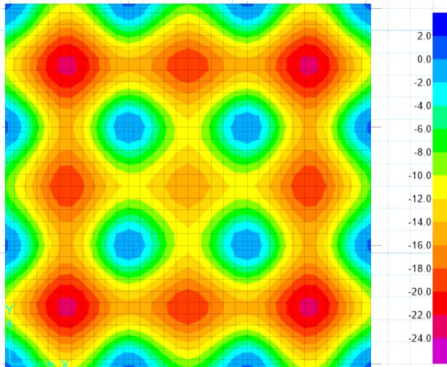
Figure 4. Long-term deflection for flat slab without drop (L=4m, LL=4.5 kN/m 2 , t=315 mm and f'_c = 21\text{MPa} )
