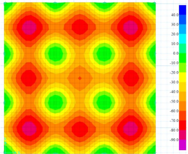
Figure 5. Long-term deflection for flat slab without drop (L=10m, LL=4.5 kN/m 2 , t=315 mm and f'_c = 21\text{MPa} )
