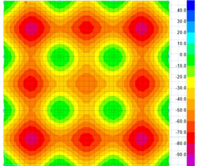
Figure 7. Long-term deflection for flat slab with drop (L=10m, LL=4.5 kN/m 2 , f'_c = 21\text{MPa} , t=290 mm and t_2=0.25t_{\text{slab}} )
